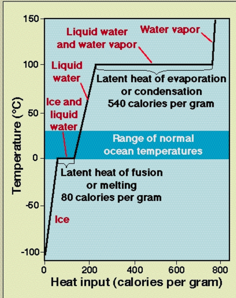
Heat Capacity of Pure Water
