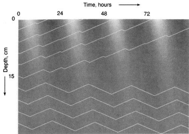
Figure 3. Computed tracks of an organism with the properties estimated for the pseudoplasmodia of the slime mold, Dictyostelium discoideum . The parameters are 0.2 cm/h rate of locomotion, 0.2 /h rate of temperature adaptation, -2^{\circ}\text{C} offset of the avoided temperature from the adapted temperature, and an unlimited temperature range of locomotion. Other features as in Figure 2.
