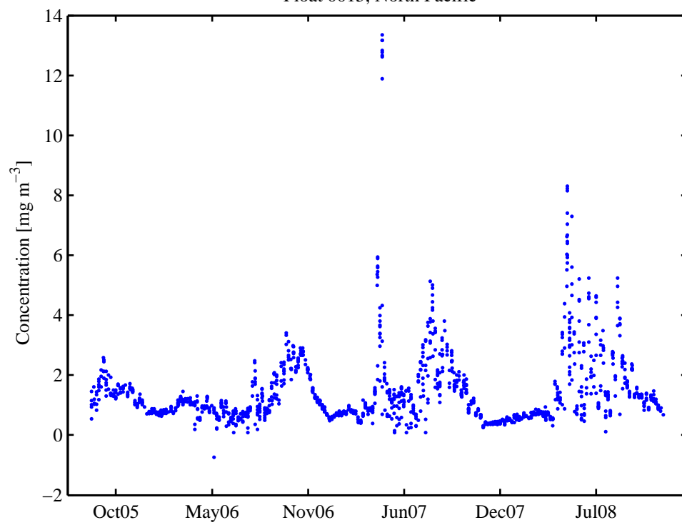
Chlorophyll Float 0015, North Pacific
