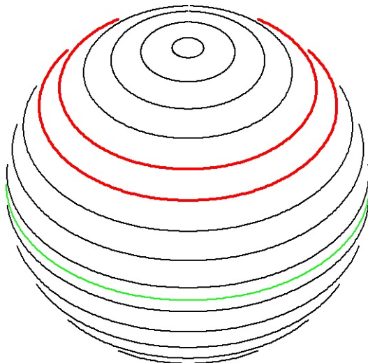
Figure 5. The EcoLight standard band layout, which has a nominal angular resolution of \Delta\theta = 10^\circ and no \phi dependence; compare with the HydroLight quad layout of Fig. 2. The red band indicates a particular 10^\circ polar angle band. The green line is the “equator” between the upper and lower hemispheres of directions.
