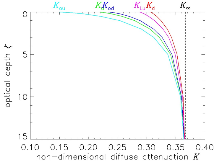
Fig. 7. Selected non-dimensional diffuse attenuation functions, as computed by the HydroLight run for Example 1. (Figure plotted by the IDL routine on HE5\examples\IDL\HE5UG_Fig7.pro.)
