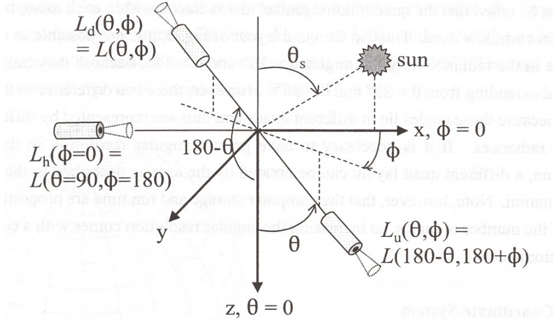
Fig 3. Coordinate system and notation conventions for radiance as used in HydroLight printout.
