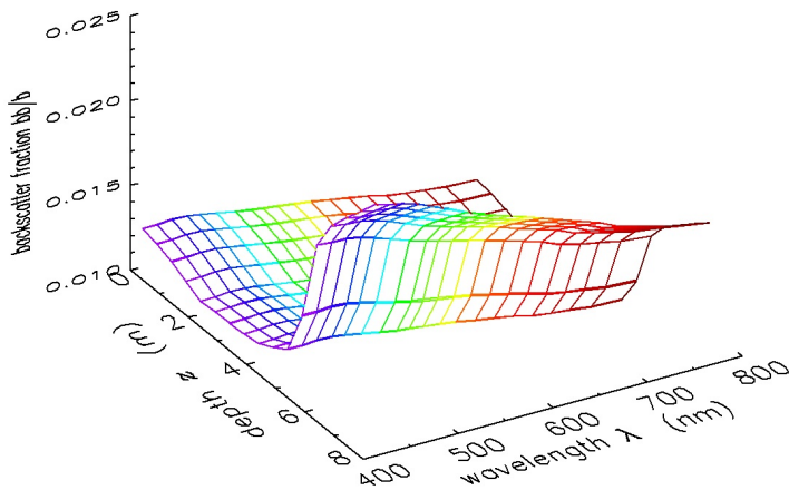
Fig. 10(f). The particle backscatter fraction b_b/b as a function of depth and wavelength, as used in Example 4.
