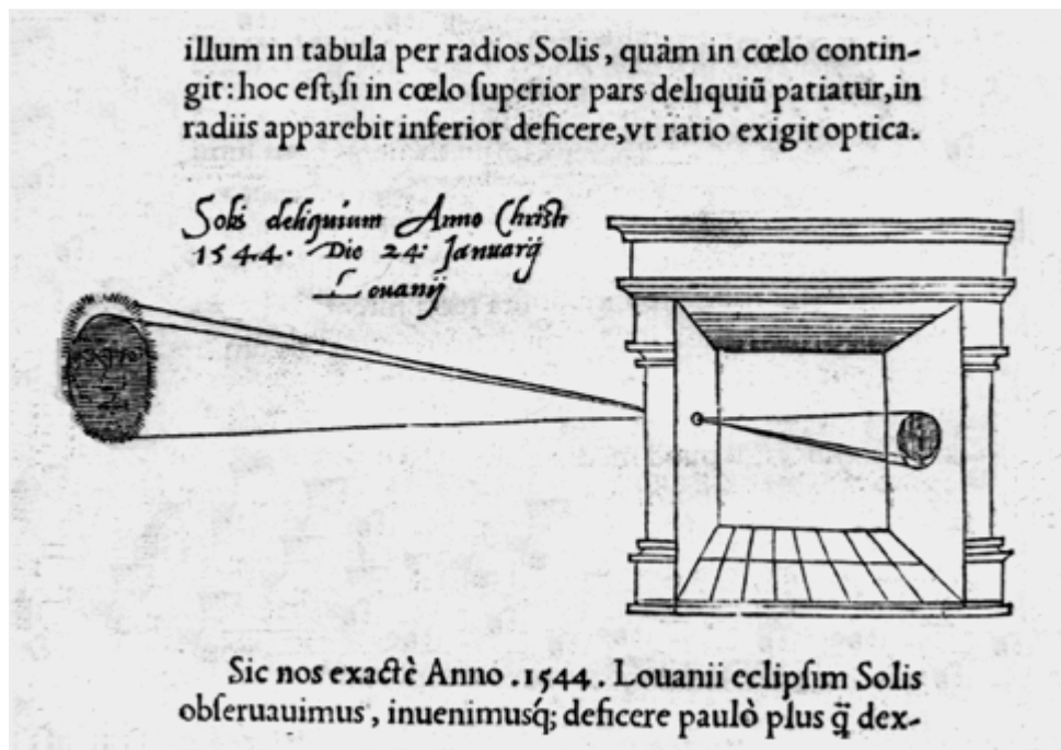
Figure 4. Example of pinhole optics from 1544. The solar eclipse is inverted in the view through the hole as it passes. Figure from:
