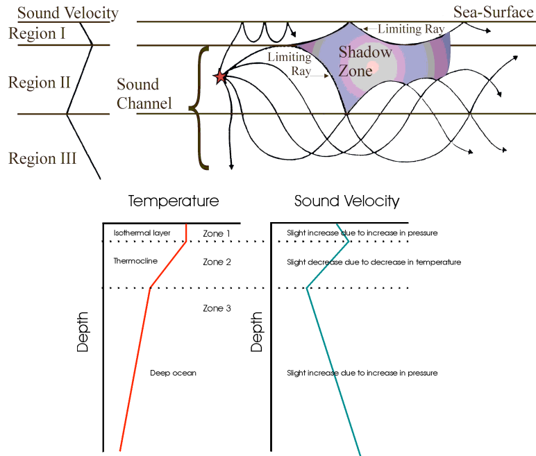
Figure 16. Sound propagation in an ocean with a typical distribution of temperature and pressure. Sound refracts as the speed of sound changes, resulting in a sound channel (SOFAR channel) where sound propagates very well. Note that here and in other layered media that vary in sound speed, sound tends to get trapped in the layers where sound velocity is slowest. It is this sound channel that allows long-distance communication between whales. From:
