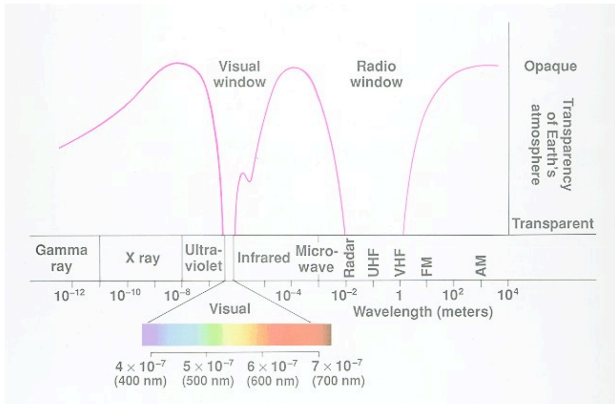
Figure 2. Light is some time referred to only a small part of the electro-magnetic spectrum, that perceived by the human eye. It is one of the regions of the spectrum where the atmosphere is almost transparent, and thus can propagate relatively unattenuated from the top of the atmosphere to the surface of the earth.
