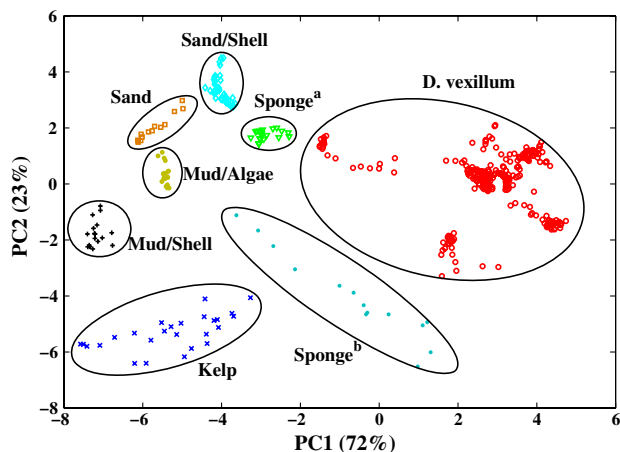
Fig. 5. (Color online) Score plot from a PCA of first derivative spectra from 490 to 557 nm. The first two principal components are plotted, accounting for 95% of the variation within the data. All substrates are easily distinguishable. The two distant D. vexillum groups were spectra collected under low illumination.
