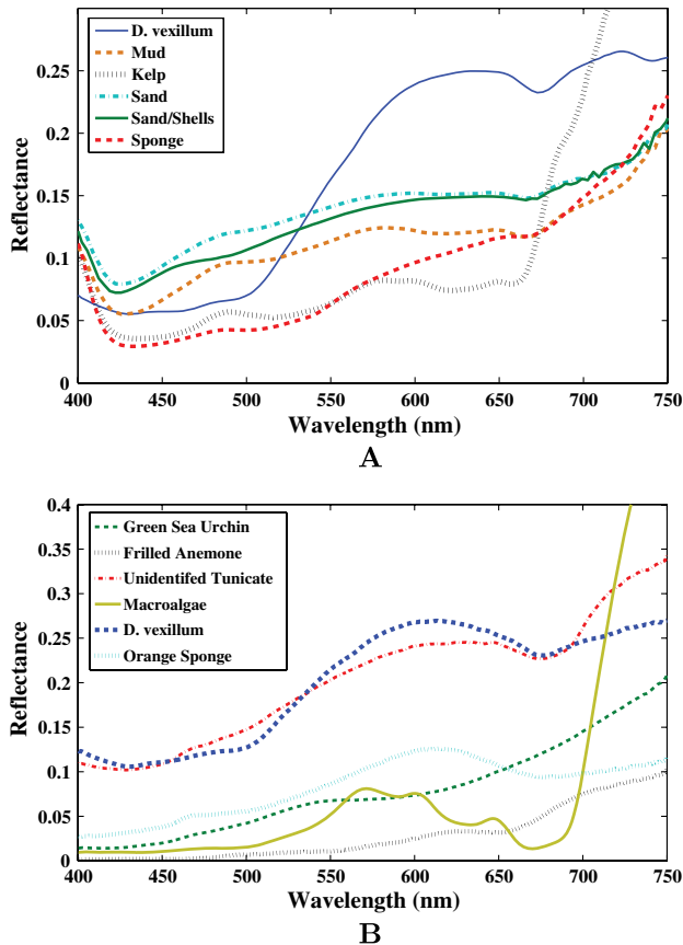
Fig. 3. (Color online) Comparison of D. vexillum spectra with other common substrates measured using (A) the HyperOCR and (B) the DiveSpec. Spectra are not area normalized and have been left as fractional reflectance ( L(\lambda)/L^*(\lambda) ) to allow for easier visual comparison.
