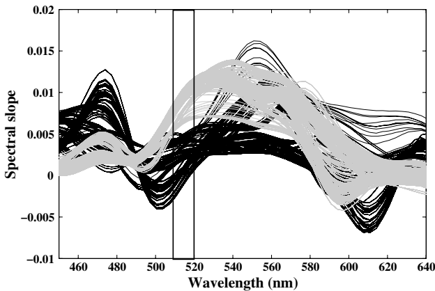
Fig. 4. First derivative spectra of D. vexillum (gray) and all other substrates measured (black). The box encloses the unique wavelengths (510–520 nm) that were used in the detection algorithm. Inside the box there is large separation between D. vexillum spectra and all other spectra collected.
