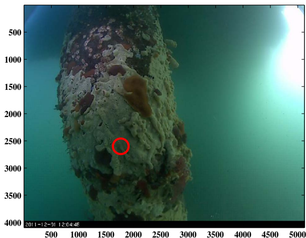
Fig. 1. (Color online) Image of D. vexillum taken by the ROV. The red circle marks the field of view of the radiometer. Axis labels denote pixel number.
