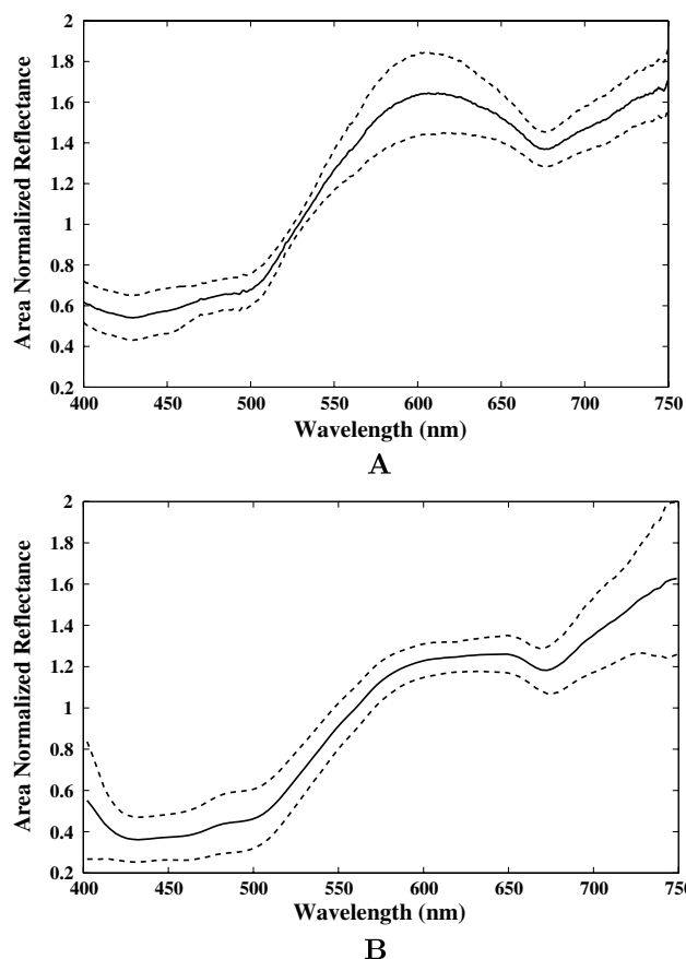
Fig. 2. (A) Mean in-situ reflectance spectra for D. vexillum using the DiveSpec ( n = 10 ) and (B) the HyperOCR ( n = 7 ). All spectra are referenced to a 95% reflectance standard. Dashed lines show 95% confidence interval.
