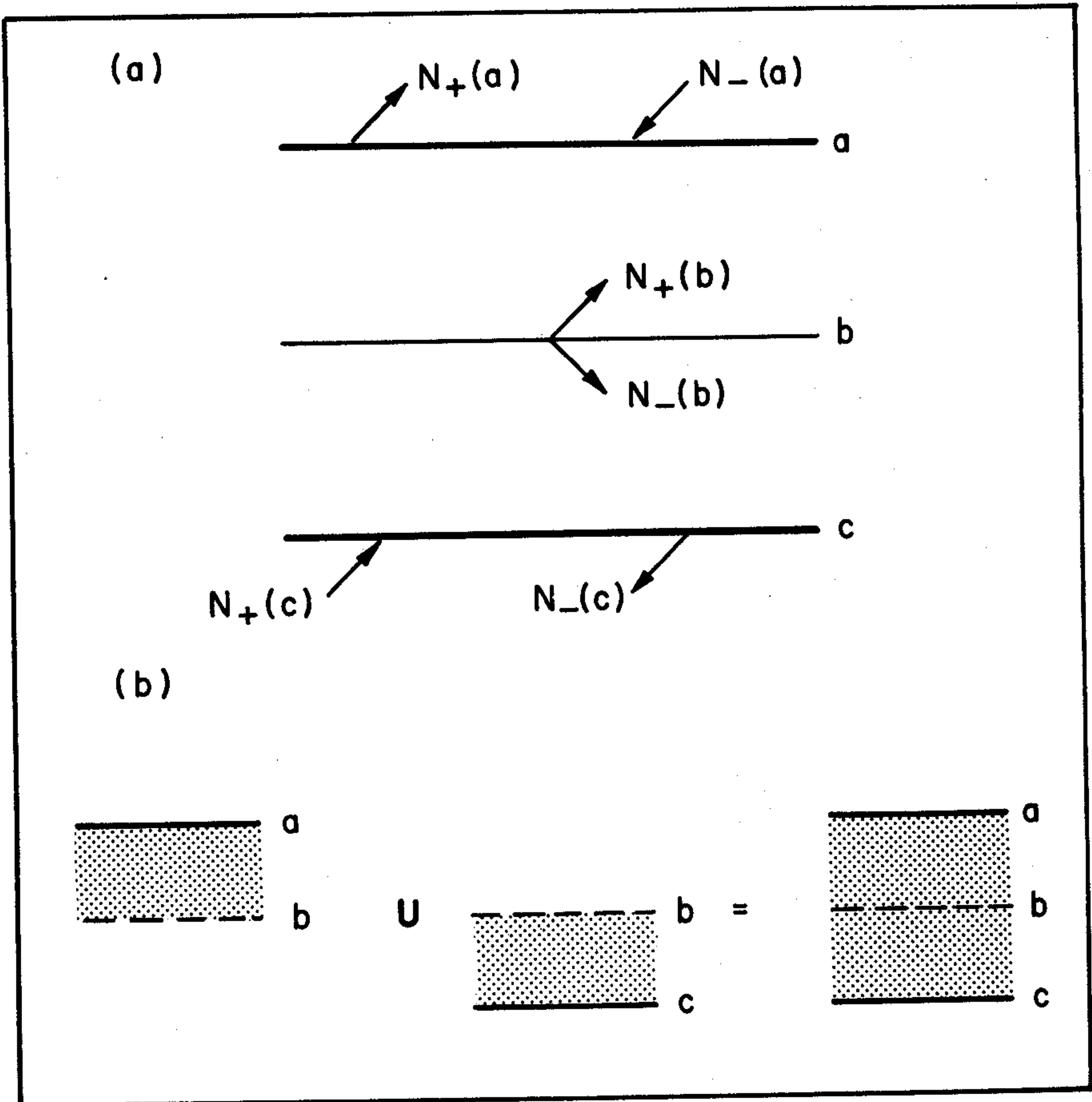
FIG. 7.2 Deriving the Partition Relations for R and T Operators.
