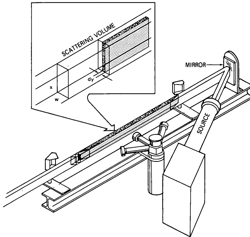
Fig. 3-3. Artist's Rendition of Modified Integrating Nephelometer.
