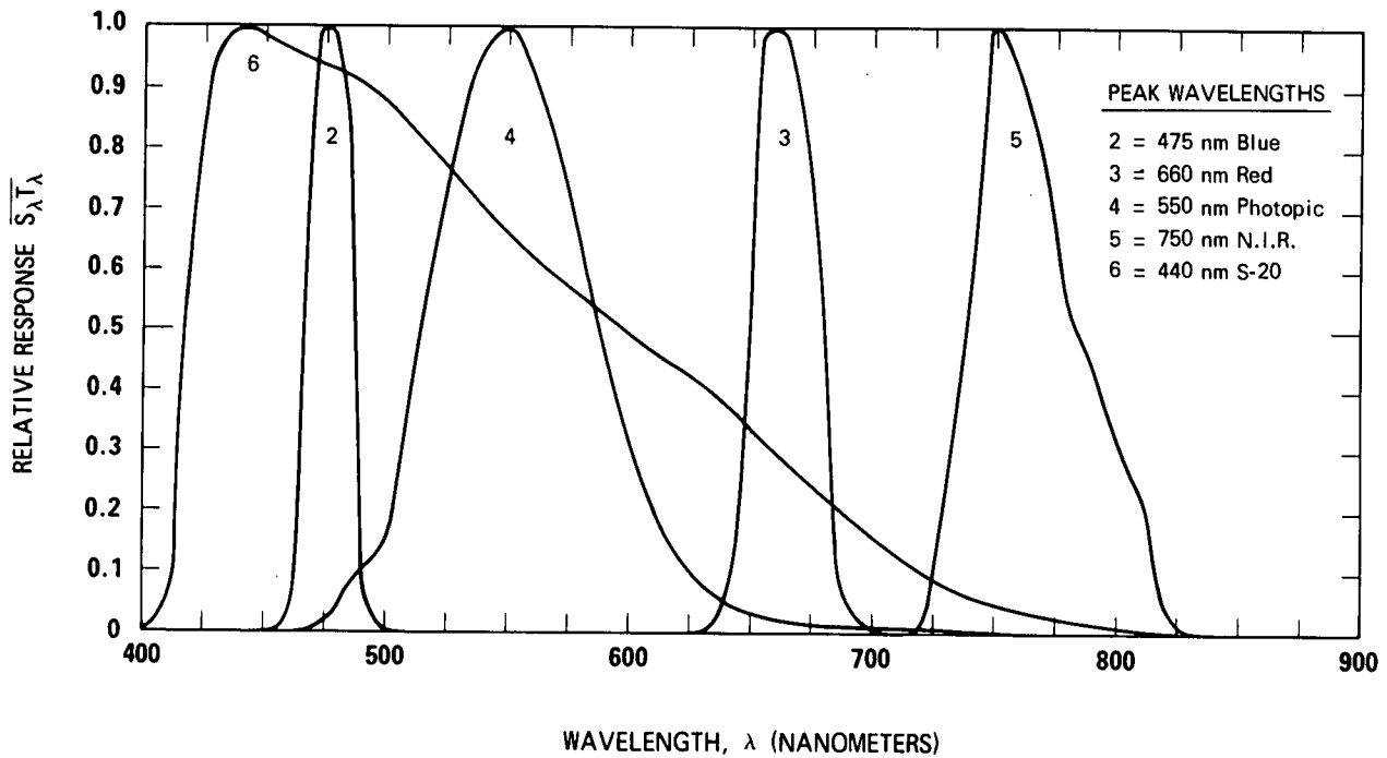
Fig. 1-2. Standard Spectral Responses – Project OPAQUE I.
