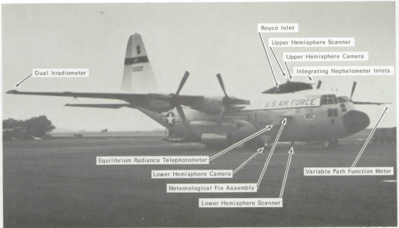
Fig. 3-1. C-130 Airborne Instrument System.
