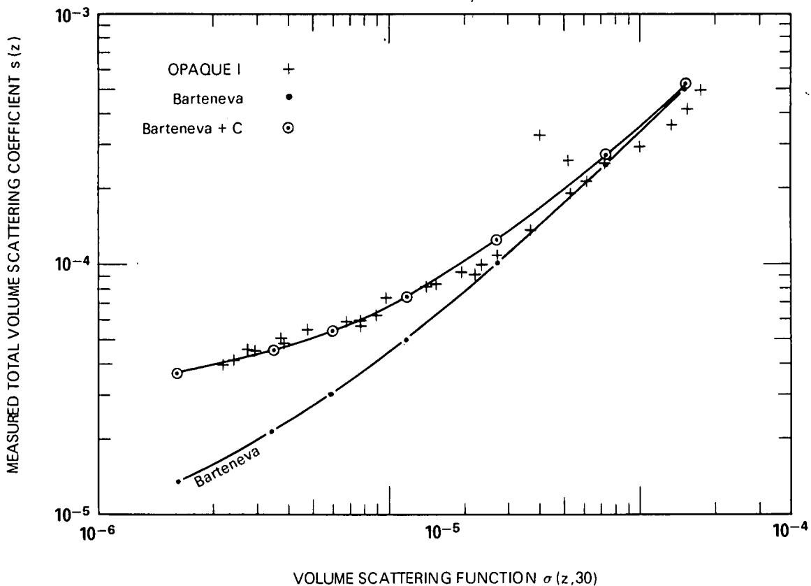
Fig. 8-5. Total Volume Scattering Coefficient as a Function of Volume Scattering Function at 30 Degrees for OPAQUE I Filter 4 Pseudo-Photopic Mean Wavelength 557 Nanometers.
