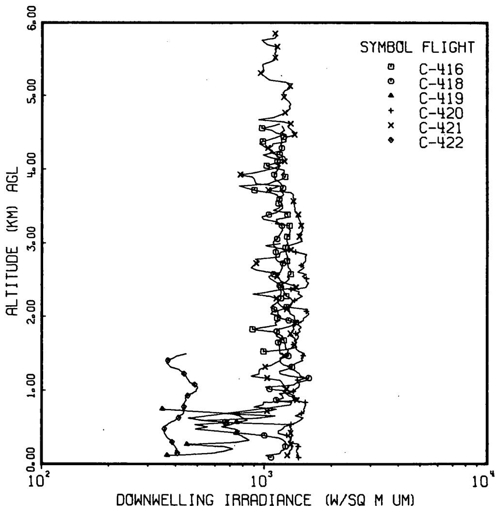
Fig. 8-14. Downwelling Irradiance for Filter 4 Pseudo-Photopic for six OPAQUE III Flights, 1 through 11 August 1977.
