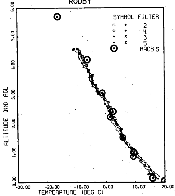
Fig. 6-2 (cont). Temperature Versus Altitude for Twelve Project OPAQUE III Flights.
