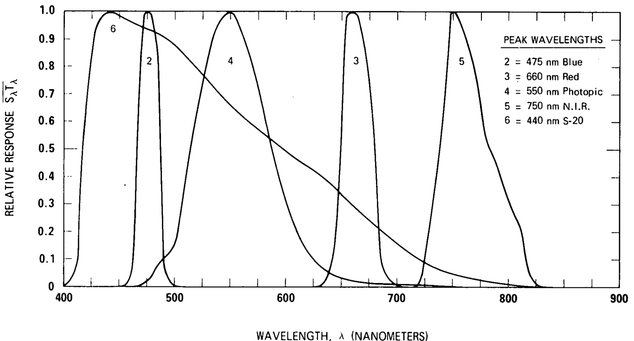
Fig. 1-2. Standard Spectral Responses - Project OPAQUE III.
