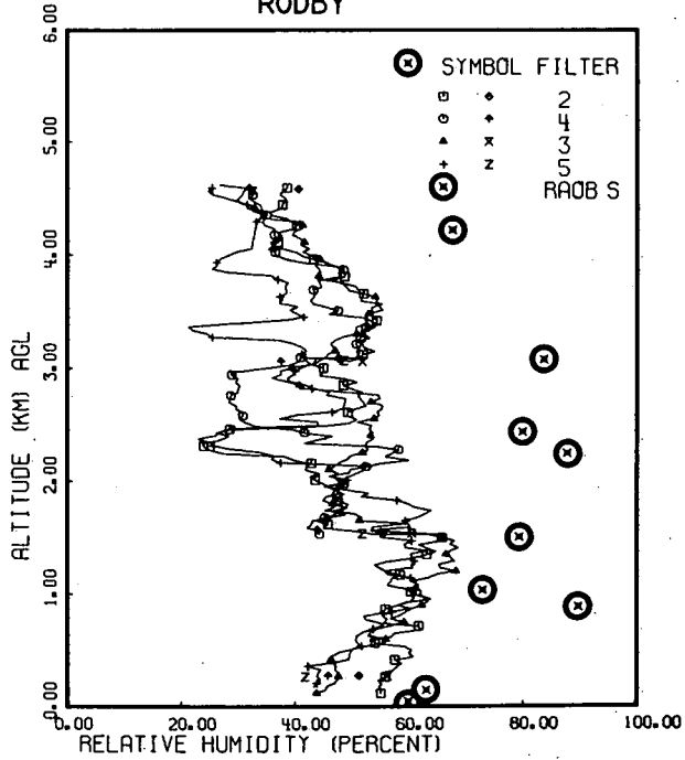
Fig. 6-3 (cont). Relative Humidity Versus Altitude for Twelve Project OPAQUE III Flights:
