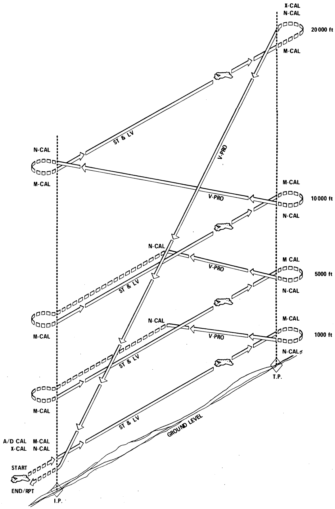
Fig. 4-1. Typical Visibility Laboratory Flight Profile
