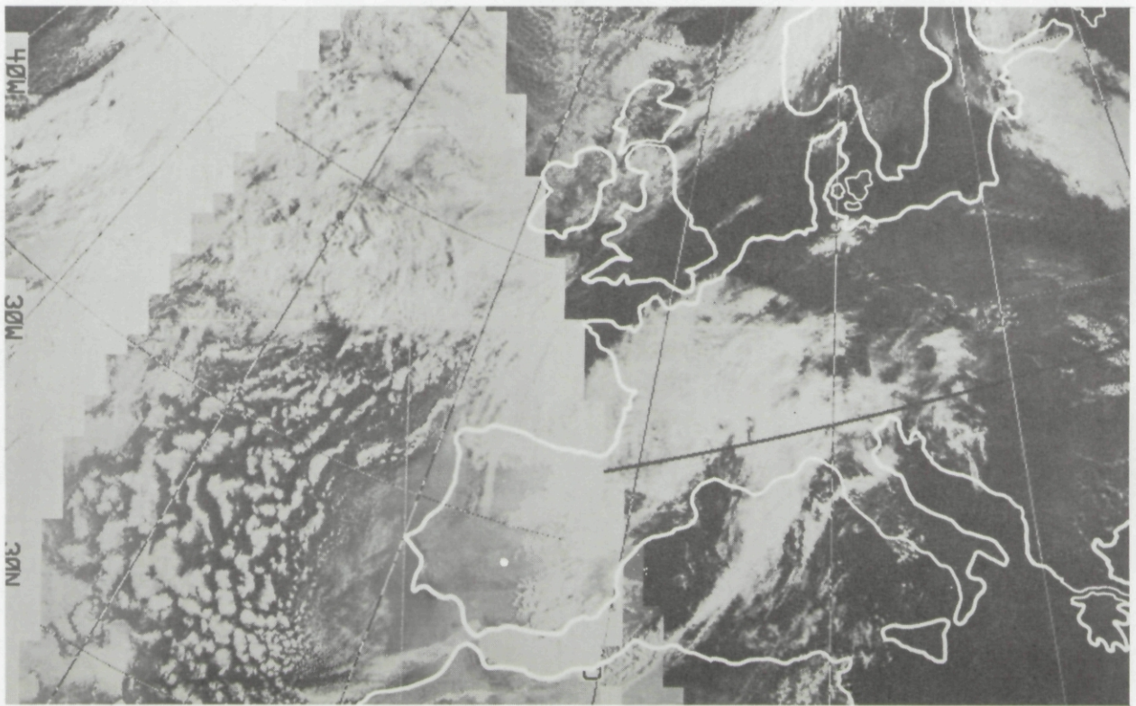
Fig. 6-4a. Satellite Photographs for 5 July 77, 1154 GMT, Reference Flts. C-410-411 (Upper) and for 30 July 77, 1309 GMT, Reference Flts. C-415 and C-416 (Lower)
