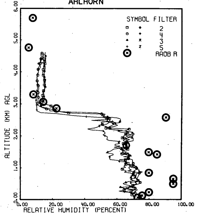
Fig. 6-3 (cont). Relative Humidity Versus Altitude for Twelve Project OPAQUE III Flights:
