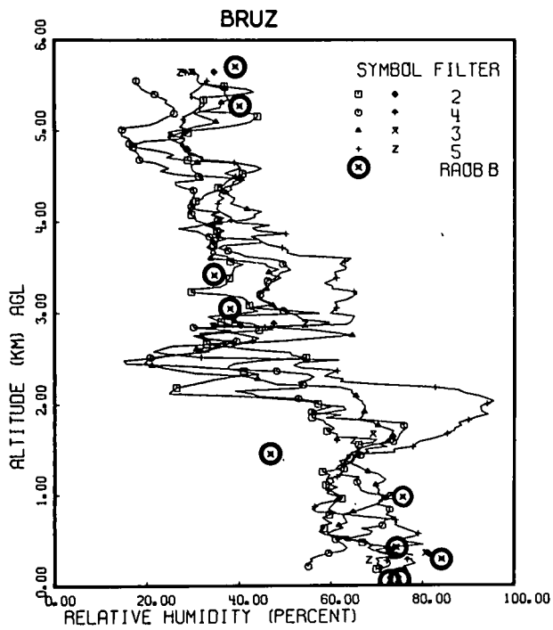
Fig. 6-3. Relative Humidity Versus Altitude for Twelve Project OPAQUE III Flights.
