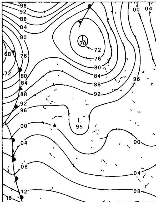
5 DECEMBER 1976 1200 GMT
