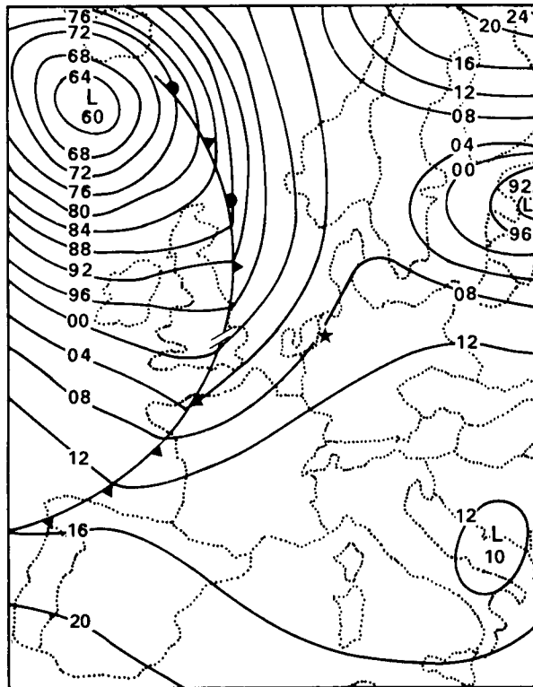
1 NOVEMBER 1976 1200 GMT
