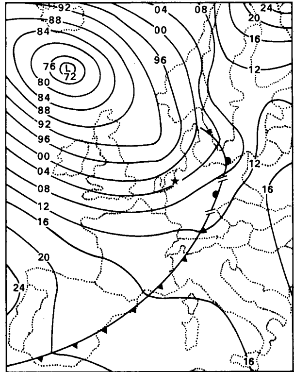
2 NOVEMBER 1976 1200 GMT
