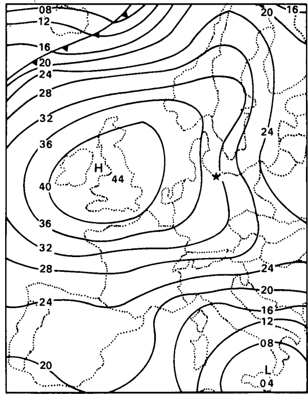
19 NOVEMBER 1976 1200 GMT
