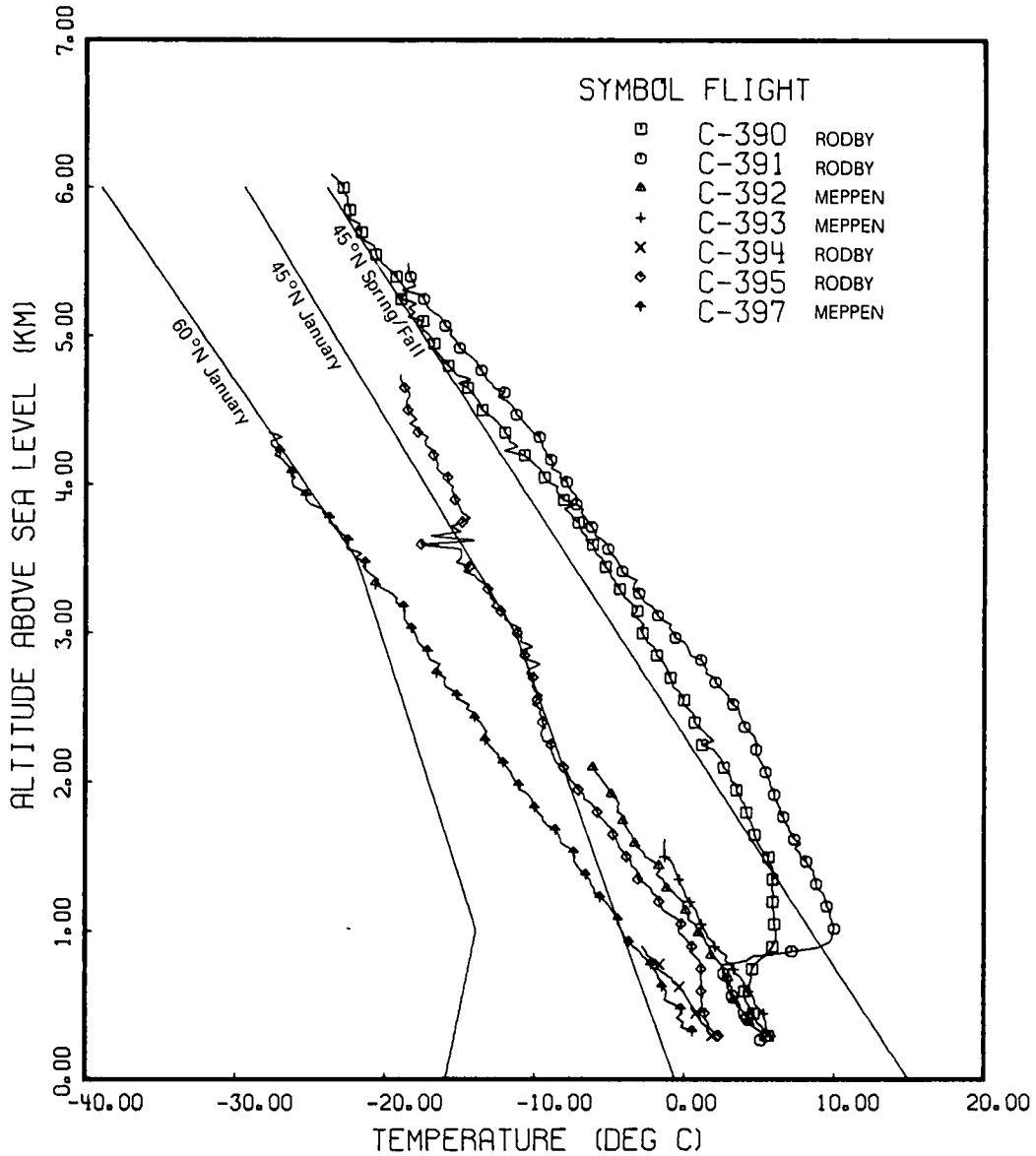
Fig. 8-1. Temperature for OPAQUE II Flights 26 October to 23 November 1976, Latitudes 53°N to 54.68°N Compared to Temperature From U.S. Standard Atmosphere Supplements (1966).
