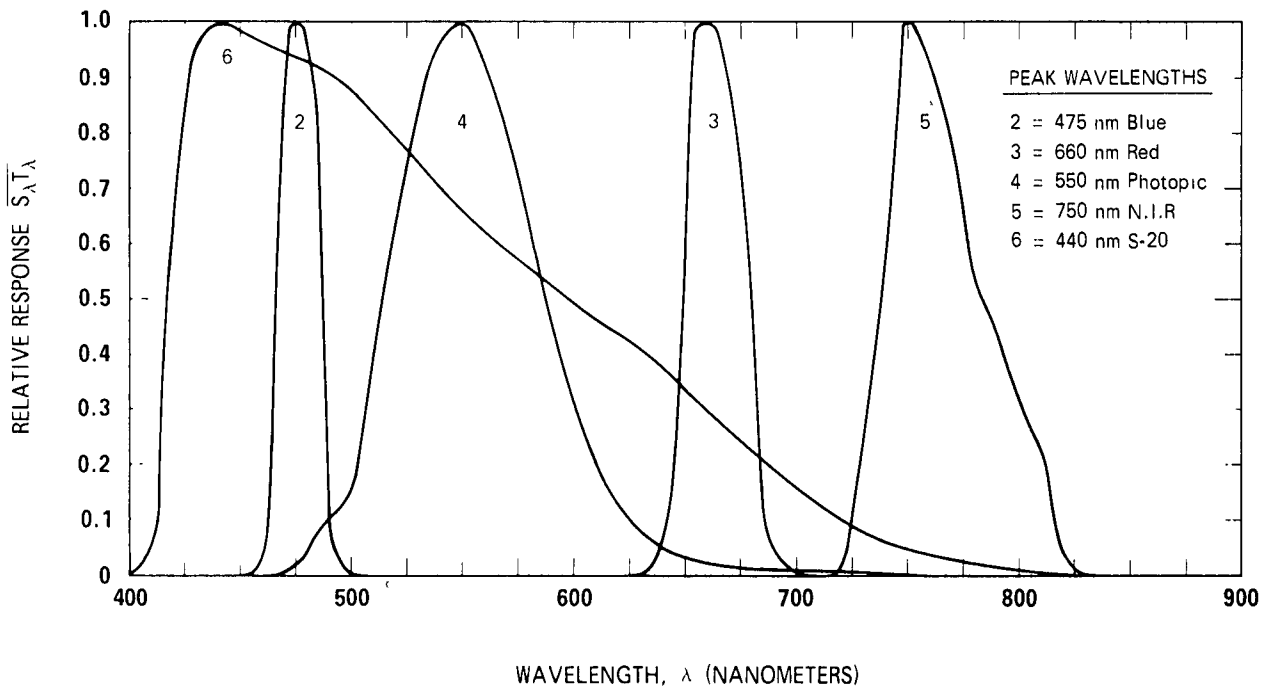
Fig. 1-2. Standard Spectral Responses – Project OPAQUE II.
