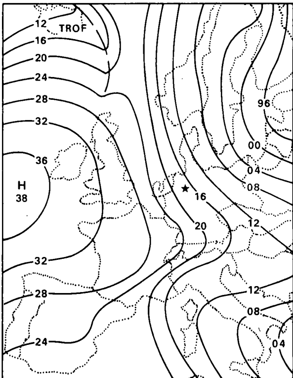
23 NOVEMBER 1976 1200 GMT
