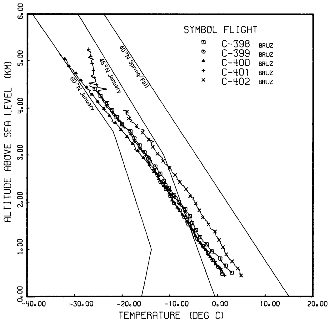
Fig. 8-2. Temperature for OPAQUE II Flights 2 to 6 December 1976, Latitude 48.02°N Compared to Temperature From U.S. Standard Atmosphere Supplements (1966).
