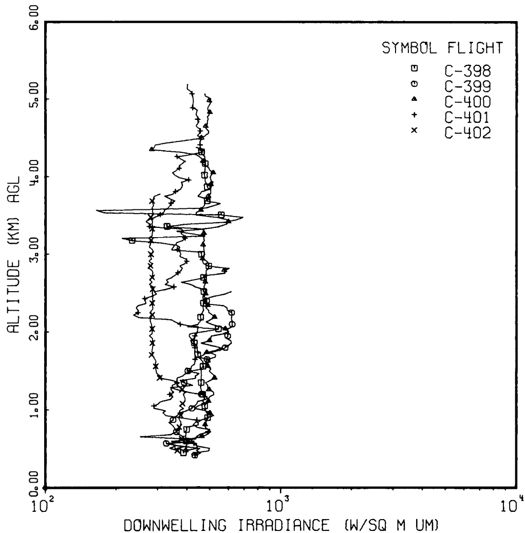
Fig. 8-14. Downwelling Irradiance for Filter 4 Pseudo-Photopic for Five OPAQUE II Flights, 2 December Through 6 December 1976.
