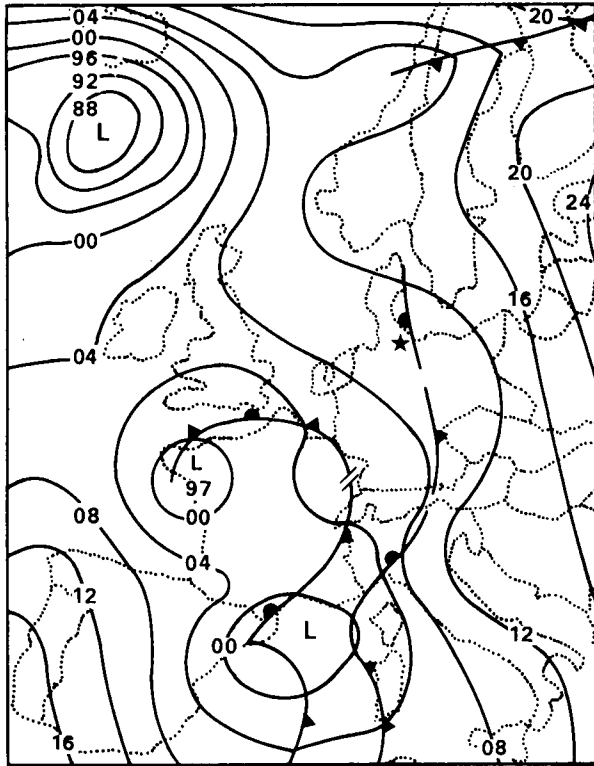
25 OCTOBER 1976 1200 GMT
