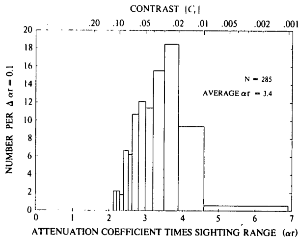
Fig. 6. Mount Washington Data Regraphed as a Function of Attenuation Coefficient Times Sighting Range \alpha r .
