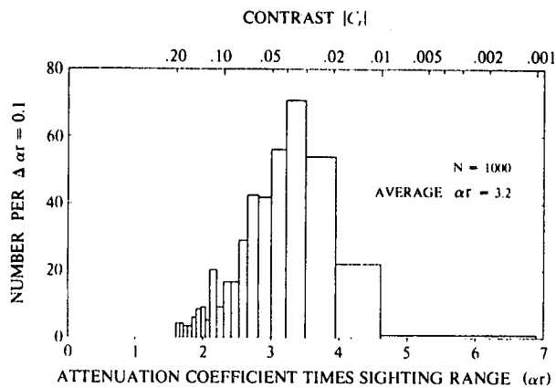
Fig. 4. Ottawa Observations Regraphed as a Function of Attenuation Coefficient Times Sighting Range \alpha r .
