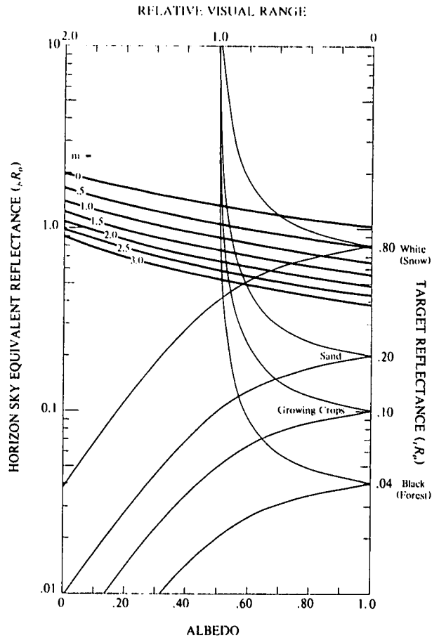
Fig. 10b. Horizon Sky Reflectance Curves with Overlay of Relative Visual Range Curves for Sample Target Reflectances.
