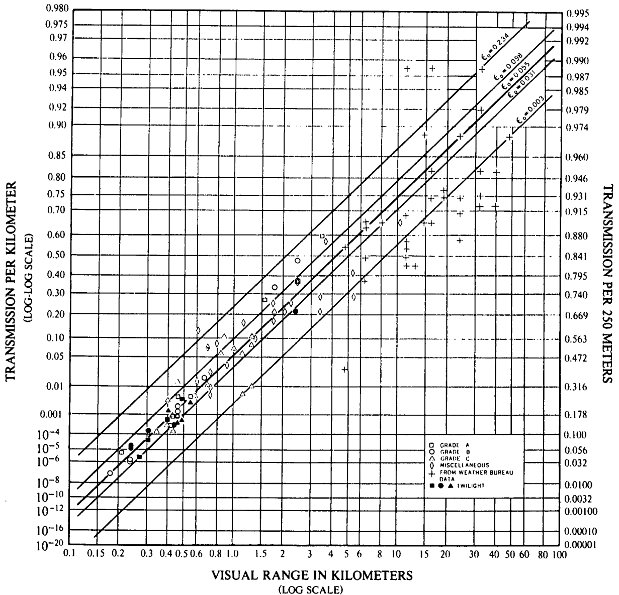
Fig. 2. Douglas and Young (1945), Figure 8, Daytime Transmissometer Calibration, \epsilon_0 = C_r .
