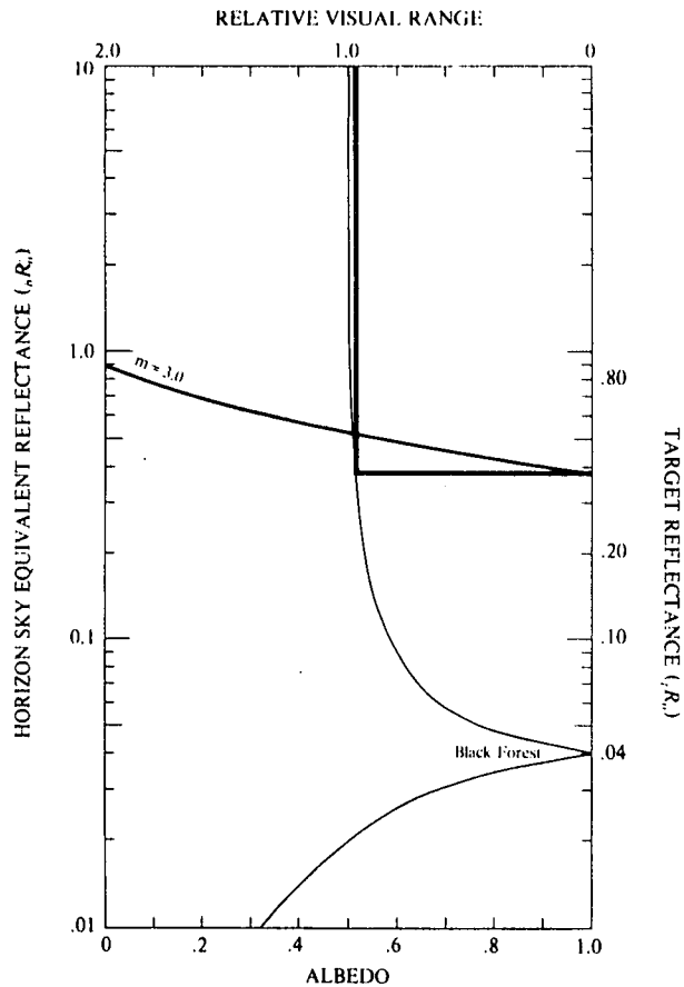
Fig. 10c. Illustration of Method of Use of Overlay Curves.
