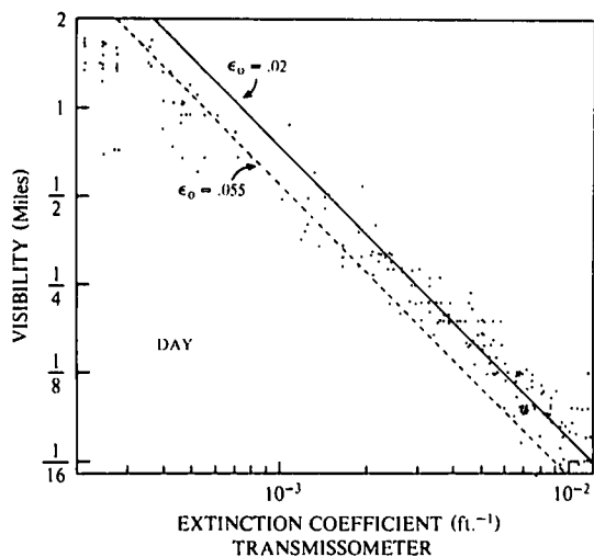
Fig. 7. Hering, et al. (1971), Figure 9, Comparison Between Transmissometer Measurements and Human Visibility Observations During the Daytime, \epsilon_0 = C_r .
