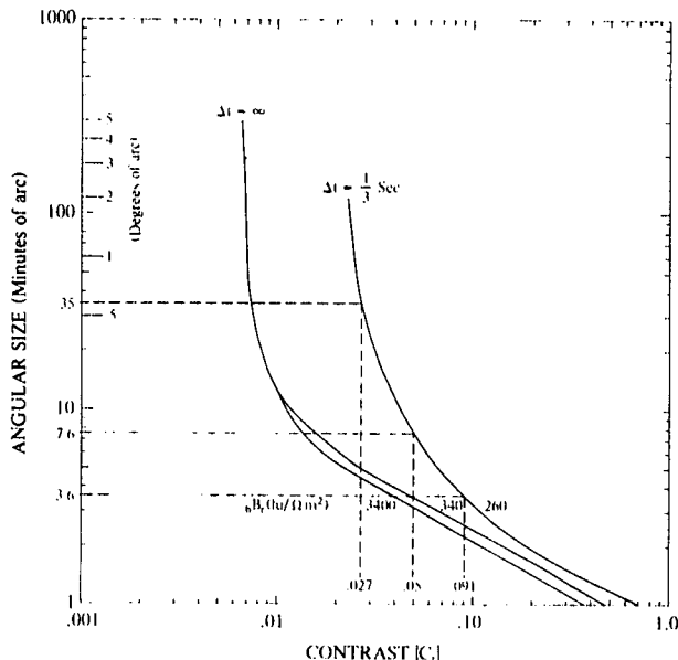
Fig. 1. Angular Size as a Function of Contrast for a 99 Percent Probability (Confidence) and a Lack of Knowledge of Target Position, of \pm 4 Degrees or More.
