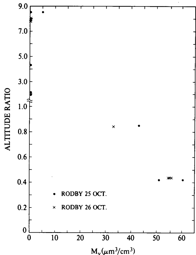
Fig. 5. The Maximum Volume in the Accumulation Mode, M_v , Measured at Rodby on October 25, 1976 (•) and on October 26, 1976 (x) as a Function of Altitude Ratio, the Ratio of the Aircraft Altitude during Measurement to the Thickness of the Mixing Layer.
