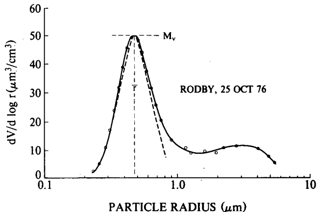
Fig. 2. The Aerosol Volume per Increment d \log r as a Function of Particle Radius for Data Taken at Rodby (Denmark) on October 25, 1976 at an Altitude of 305m above the Sea Surface (solid line). The mode radius, \bar{r} , and maximum, M_v , of the volume distribution accumulation mode are shown. A log-normal distribution with \bar{r} = 0.45\mu m and standard deviation \sigma = 0.13 is shown (dashed line) for comparison.
