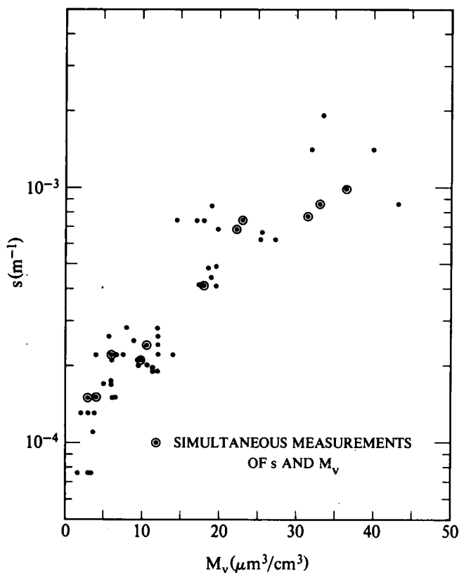
Fig. 4. The Volume Scattering Coefficient, s , for the Wavelength 0.664\mu m as a Function of the Maximum Volume, M_v . Cases where s and M_v were measured simultaneously are circled.
