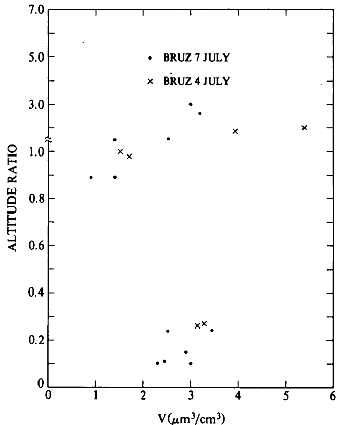
Fig. 7. The Volume Concentration of Particles in the Coarse Particle Mode, V , as a Function of Altitude Ratio for Data Collected at Bruz on July 7, 1977 (·) and on July 4, 1977 (x).
