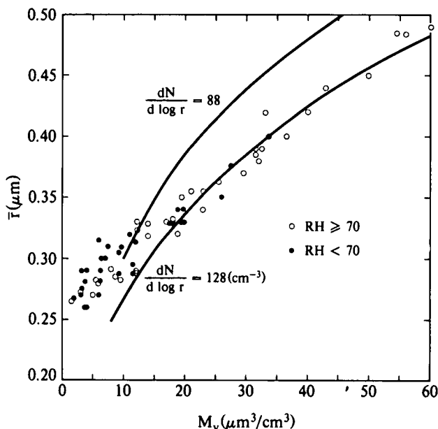
Fig. 3. The Mode Radius, \bar{r} , as a Function of the Maximum Volume, M_v , for all Data Collected within the Mixing Layer. Curves of dV/d\log r for constant particle number density, dN/d\log r , (solid lines) show the \bar{r}^3 dependence of M_v . Data for which the relative humidity is greater than or equal to 70% are indicated by the open circles.
