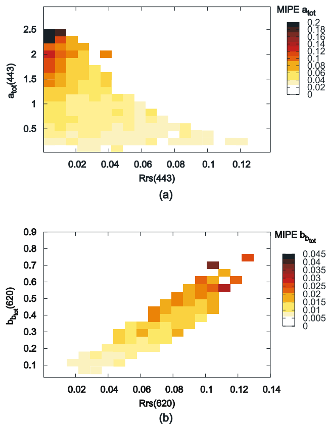
Figure 15. Maps of minimum inverse problem error ( \text{m}^{-1} ) expressed in terms of IOPs versus Rrs: (a) for a_{\text{tot}} (443) ( \text{m}^{-1} ) and (b) for b_{\text{tot}} (620) ( \text{m}^{-1} ).
