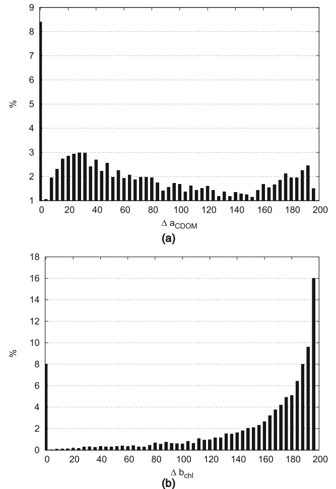
Figure 11. Distributions of ambiguity distances (dimensionless) within DPC_{K2} : (a) \Delta a_{CDOM} and (b) \Delta b_{chl} .
