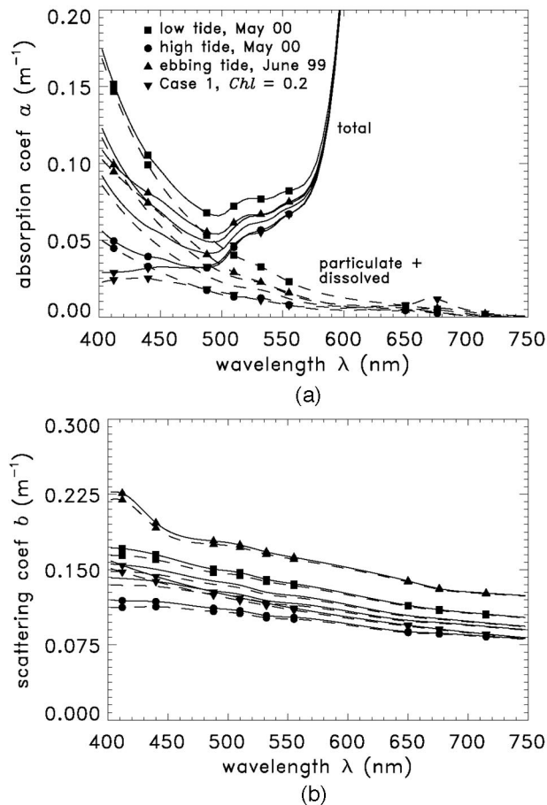
Fig. 4. Measured ac-9 (a) absorption and (b) scattering spectra. The solid curves include pure water; symbols are at the ac-9 wavelengths.
