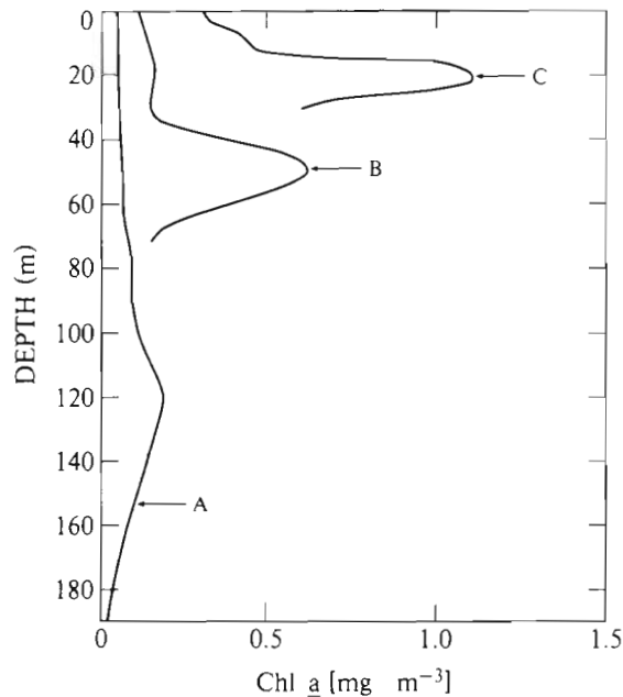
Fig. 1 Typical chlorophyll profiles plotted as function of geometrical depth (Cullen and Eppley, 1980): (A) North Pacific Central Gyre, near 28° N, 155° W (from Beers et al., 1975); (B) SCBS 15, Sta 205; (C) SCBS 7, Sta. 102
