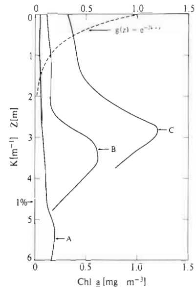
Fig. 2. Same profiles as in Fig. 1 plotted as function of attenuation lengths of PAR ( K_{PAR} \cdot Z ). The remote sensing weighting function, g(Z) , is shown as dashed curve. Depth of euphotic zone, taken as 1% PAR level, is indicated by an arrow on vertical scale
