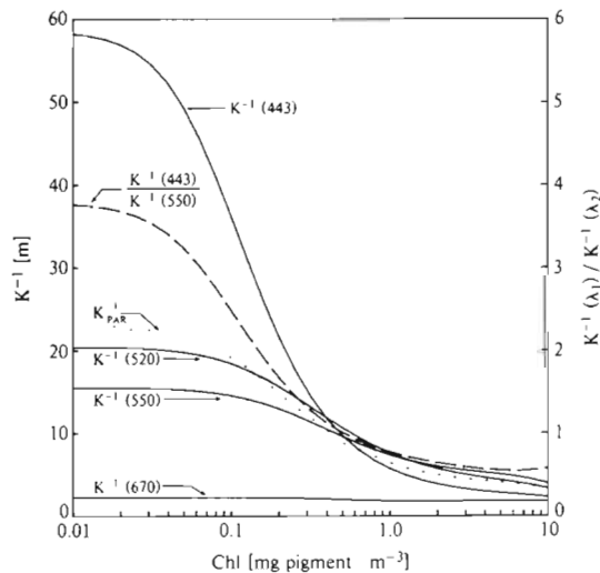
Fig. 3. Penetration depth, Z_{(H)} \approx K^{-1} (m), versus chlorophyll concentration, C ( \text{mg} \cdot \text{m}^{-3} ) as derived from an optical classification model (Smith and Baker, 1978b; Baker and Smith, 1981). Penetration depth calculated for 4 CZCS spectral bands K_{\lambda}^{-1} and for total photosynthetically available radiant energy, K_{PAR}^{-1} . Scale on right ordinate gives ratio of penetration depth in blue band to that in the green, K_{443}^{-1}/K_{550}^{-1} .
