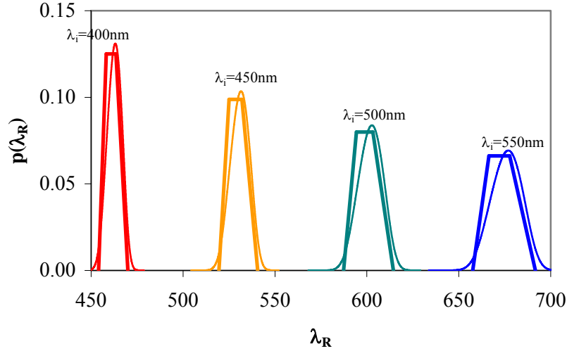
Figure 7 – Raman emission probability functions for 400, 450, 500, and 550 nm. The piecewise-linear profiles are computed from Table 4, and the smooth functions are reproduced from Mobley [21].
