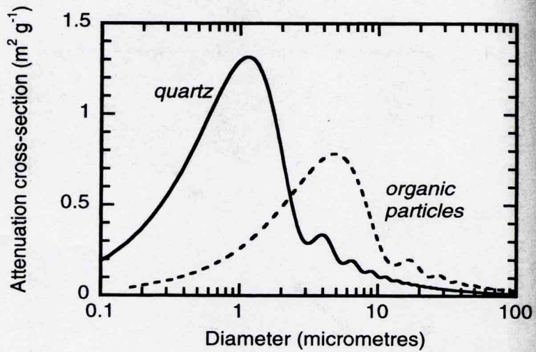
Figure 5. Attenuation Cross-Section (attenuation per unit mass) of a Suspension of Spherical Particles as a Function of Their Diameter (Davies-Colley et al. , 1993).
