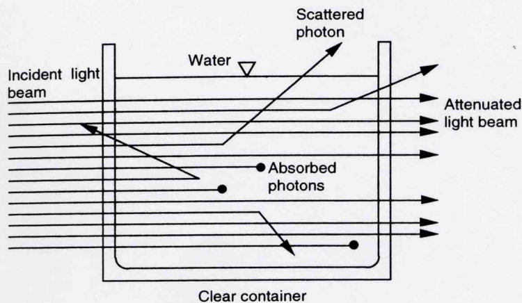
Figure 1. Schematic Diagram Showing the Paths of Representative Photons Interacting With Water by the Processes of Absorption and Scattering (Davies-Colley et al. , 1993).
