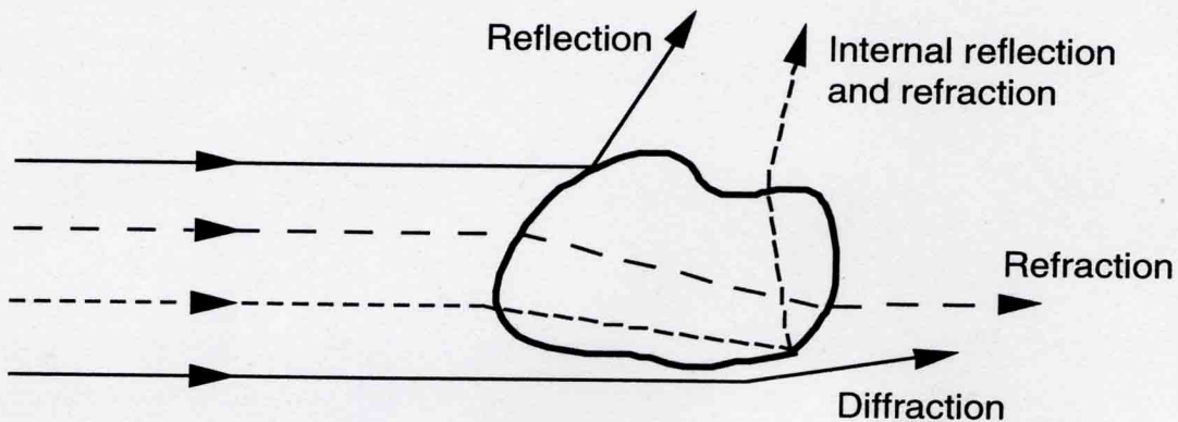
Figure 4. Schematic of the Scattering of Light by a Suspended Sediment Particle Via the Processes of Reflection, Refraction, and Diffraction (Davies-Colley et al. , 1993).
