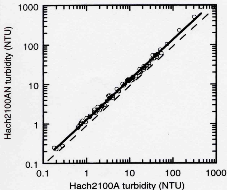
Figure 3. Comparison of Turbidity Measured Simultaneously Using Two Different Nephelometers. A Hach 2100A nephelometer (vertical incident light beam) and its modern replacement, a Hach 2100AN ratio nephelometer (horizontal incident light beam) were used side-by-side on the same batch of 77 New Zealand river water samples. (Average ratio = 1.3, coefficient of variation of the ratio = 12 percent.)
