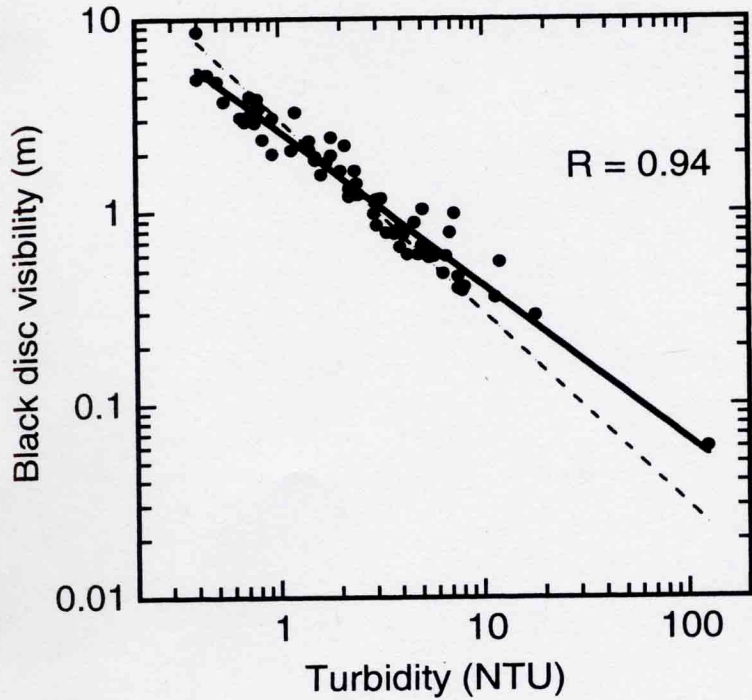
Figure 7. Black Disc Visibility and Nephelometric Turbidity (Hach 2100A) at 64 River Sites in New Zealand. Data are medians for sites in New Zealand's National Rivers Water Quality Network (Smith et al. , 1997). Each site is sampled monthly, and six years of data were used for the analysis, that is, each point represents the median of 72 samples. Both the power law fit to the data (solid line) and a simple inverse ( y_{BD} = 3.02/T ) (dashed line) are shown.
