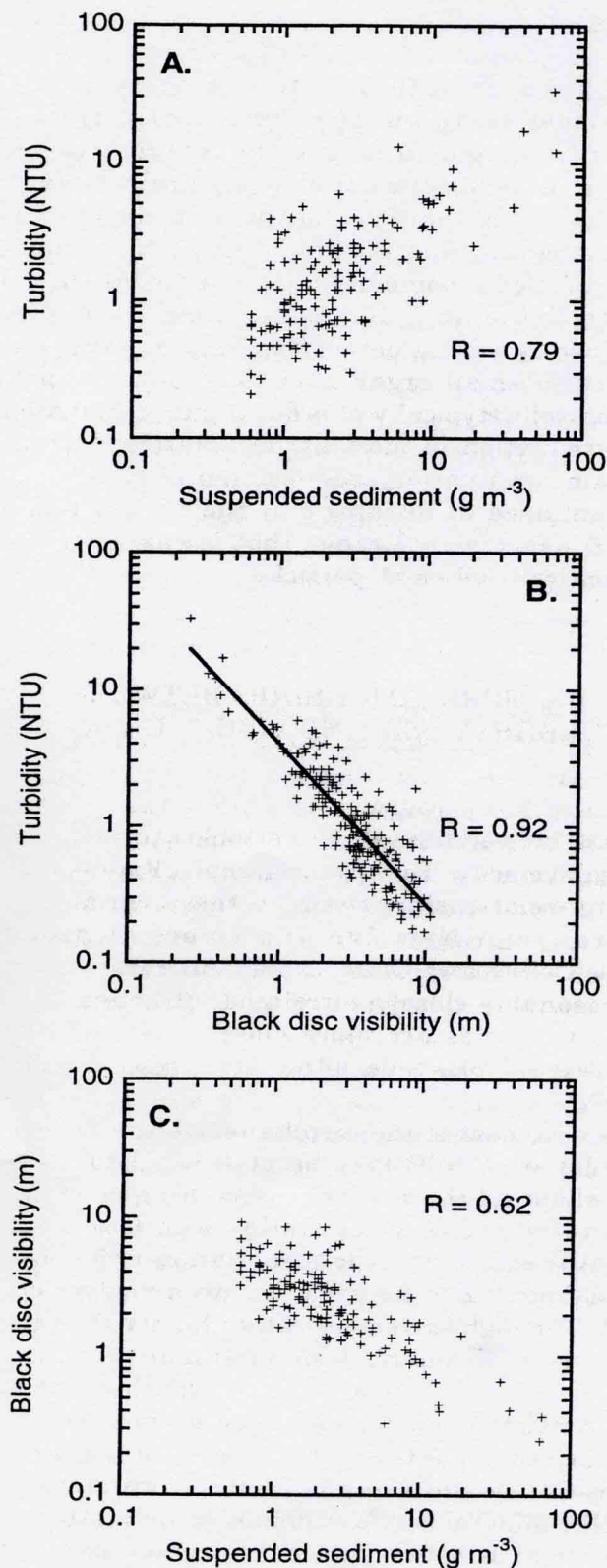
Figure 6. Mutual Relationships of Visual Clarity, Turbidity (Hach 2100A) and Suspended Sediment Concentration in 97 New Zealand Rivers (each river site sampled up to three times- n = 274 in total). Panel A. Turbidity Versus Suspended Sediment, B. Turbidity Versus Black Disc Visibility, and C. Black Disc Visibility Versus SSC. (Davies-Colley and Close, 1990).
