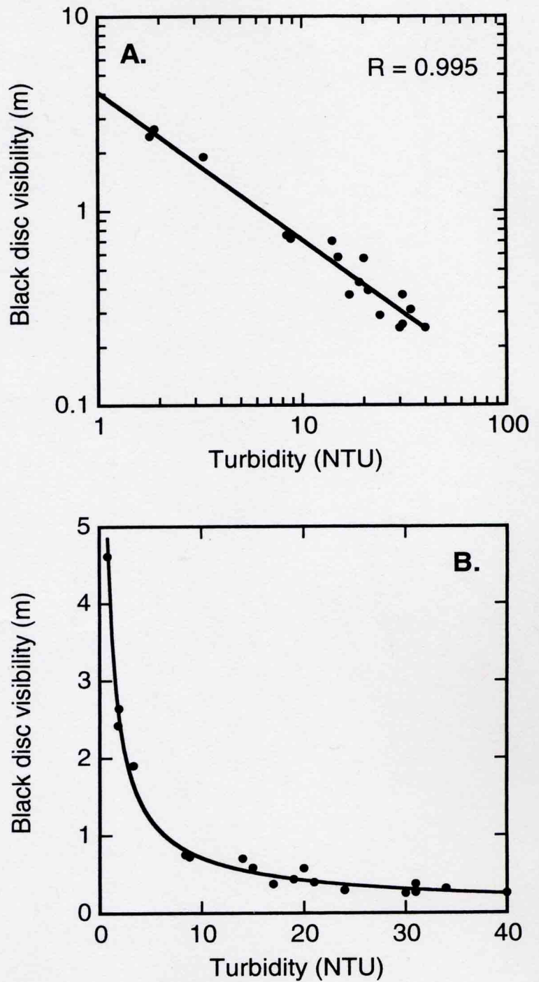
Figure 8. Black Disc Visibility Versus Turbidity (Hach 2100AN nephelometer) for 16 Sites in the Esopus and Schoharie Catchments, in the Catskill Region of New York (New York City Department of Environmental Protection, unpublished data). A. Logarithmic Scales, B. Same Data on Linear Scales. The data is well fitted ( r = 0.995 ) by a power law: y_{BD} = 4.09T^{-0.76} .
