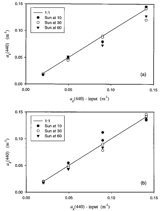
Fig. 11. (a) Inversion-derived gelbstoff absorption at 440 nm compared with input values for simulated data with 5 m/s of wind. The Y value used in inversion was random (see text). (b) As in (a) with 10 m/s of wind.
