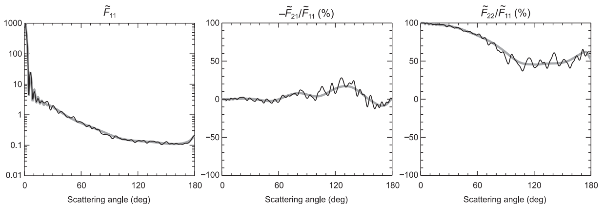
Fig. 44. Elements of the dimensionless scattering matrix computed for an imaginary spherical volume populated by N = 200 particles with m = 1.32 . Black curves: the multi-particle configuration is fixed and the results are averaged over a range of wavelengths such that k_1R varies from 47.5 to 52.5 and k_1r varies from 3.8 to 4.2. Gray curves: the results are averaged over the uniform orientation distribution of the multi-particle configuration at a single wavelength such that k_1R = 50 and k_1r = 4 .
