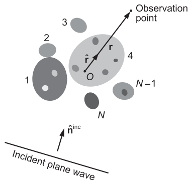
Fig. 6. Standard electromagnetic scattering problem. The fixed finite scattering object consists of N distinct and potentially inhomogeneous components. The shaded areas collectively represent the interior region V_{\text{INT}} , while the unshaded exterior region V_{\text{EXT}} is unbounded in all directions.
