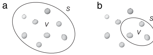
Fig. 11. Energy budget of a finite volume enclosing (a) the entire scattering object or (b) a part of the object.
