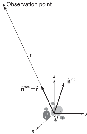
Fig. 7. Scattering in the far zone of the object.
