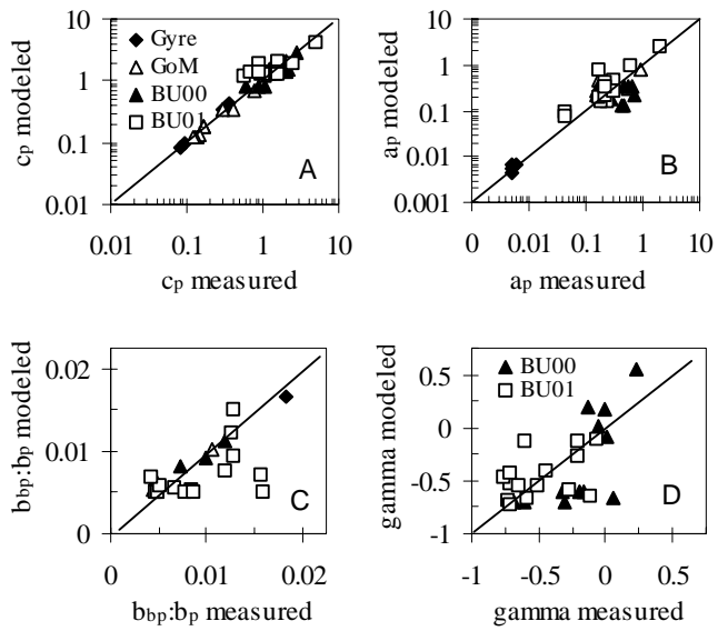
Figure 2. Relationship between measured and modeled optical properties. Particulate attenuation (A) and absorption coefficient (B) at 440nm, particulate backscattering ratio at 650nm (C; 532 nm for gyre and GoM), and slope of the particulate attenuation spectrum ( \gamma , D).
