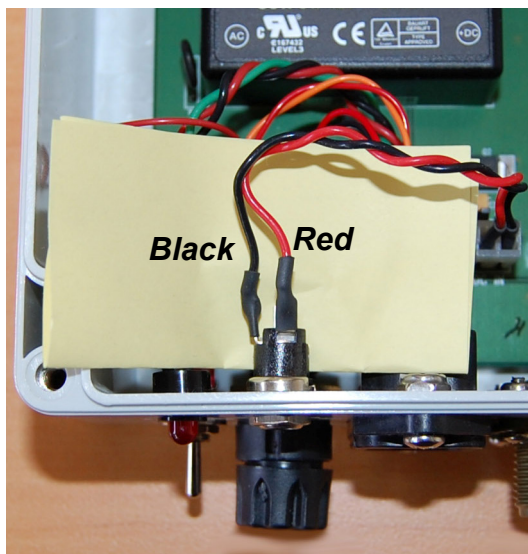
DC In Wiring Detail (paper inserted to clearly show wiring to DC In ): Correct wiring is black wire on left, red wire on right
