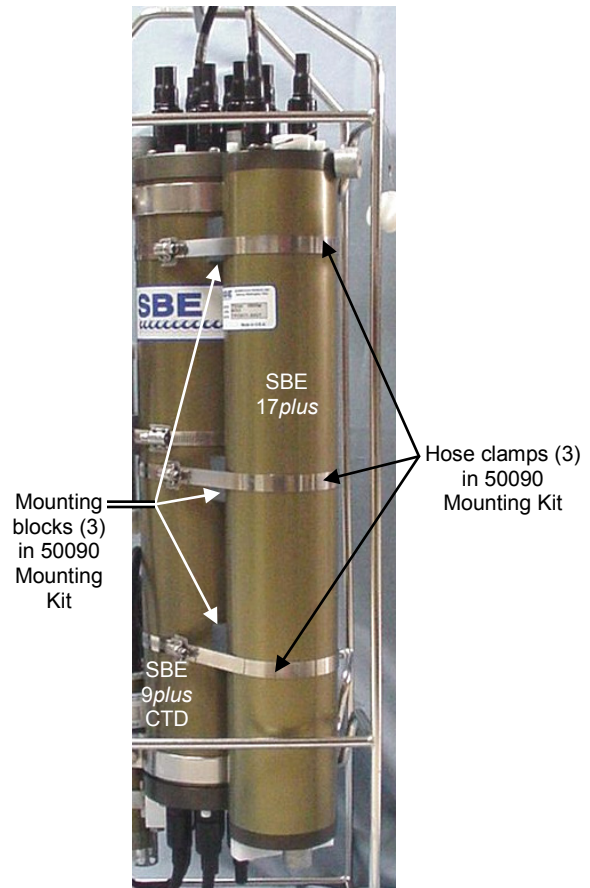
50090 Mounting Kit (shown installed on 17plus); kit also includes Teflon tape for preventing contact of stainless steel clamps to aluminum housing
