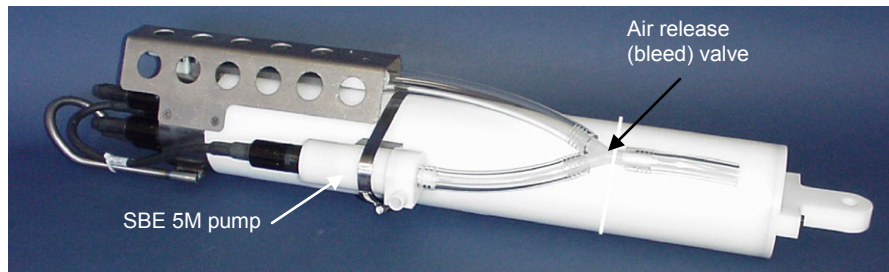
Standard Configuration - SBE 19plus V2 (plastic housing) with SBE 5M pump (plastic housing) & associated plumbing (plumbing configuration shown for 19plus V2 to be deployed in vertical orientation)
