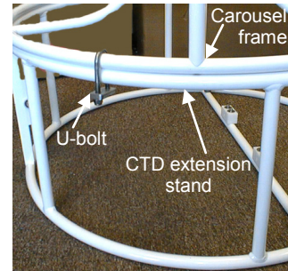
CTD extension stand (for attaching to Carousel frame with included U-bolts)
