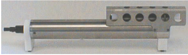
SBE 37-SM (AF24173 Anti-Foulant Devices installed at Sea-Bird)
