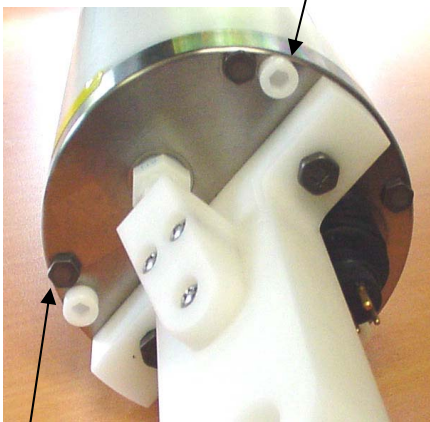
Titanium hex-head screw (typical, 4 places)
