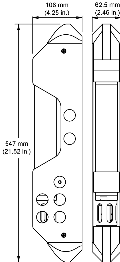
39-IM with Fairing (shown with external thermistor)
