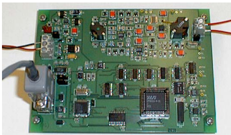
Surface Inductive Modem (SIM) PCB (1 per mooring, optional)
