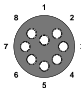
Figure A-6 - Subconn ® MCBH8F Female Face View
