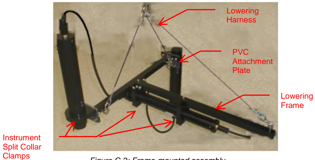
Figure C-2: Frame-mounted assembly
