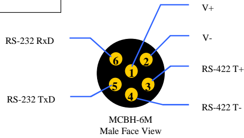
Figure A-4: HyperPro Instrument Body
