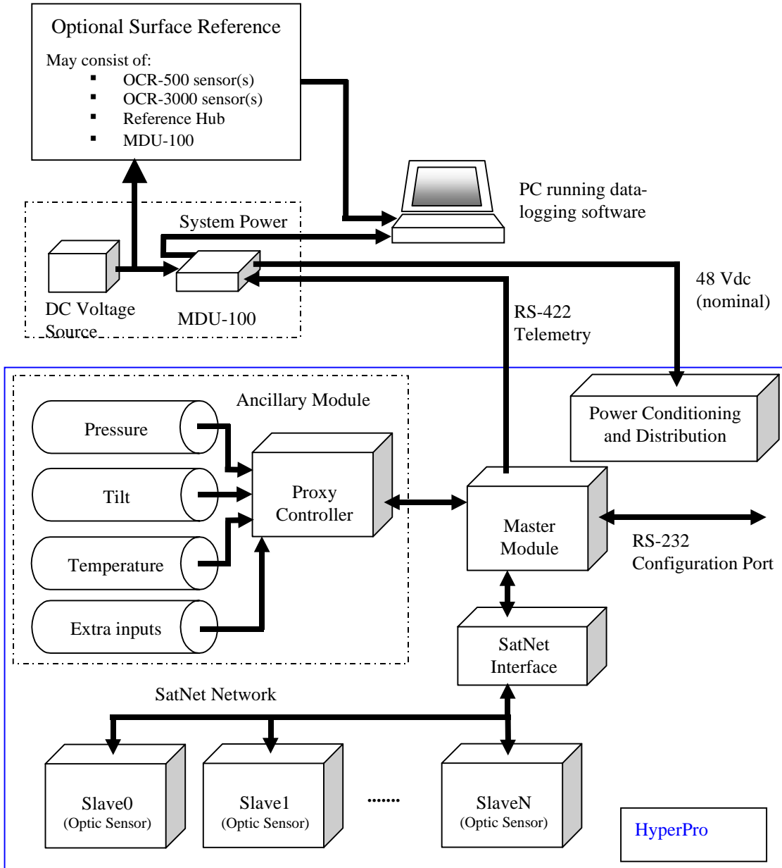
Figure A-2: HyperPro System Block Diagram
