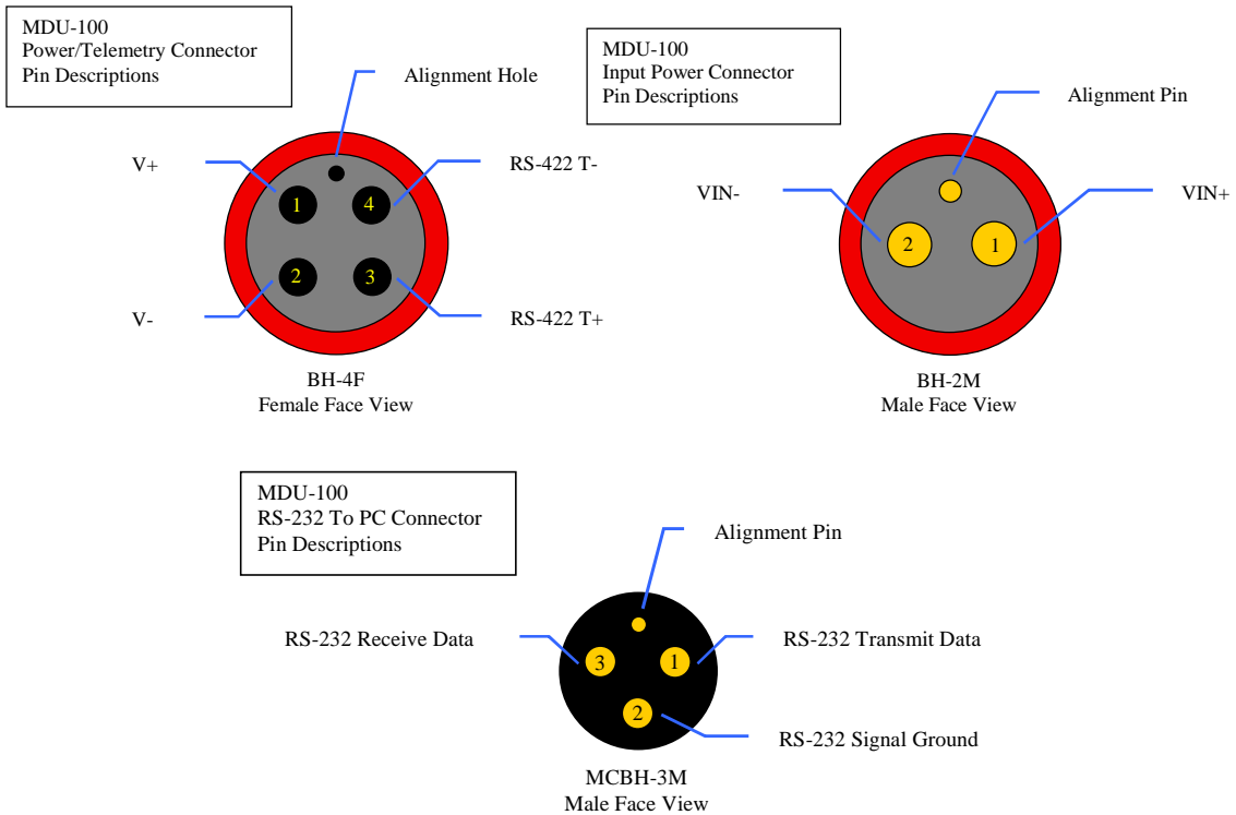
Figure A-7: MDU-100 Deck Unit
