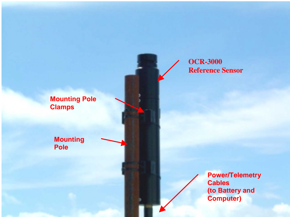
Figure A-10: Standalone OCR-3000 Reference Sensors
