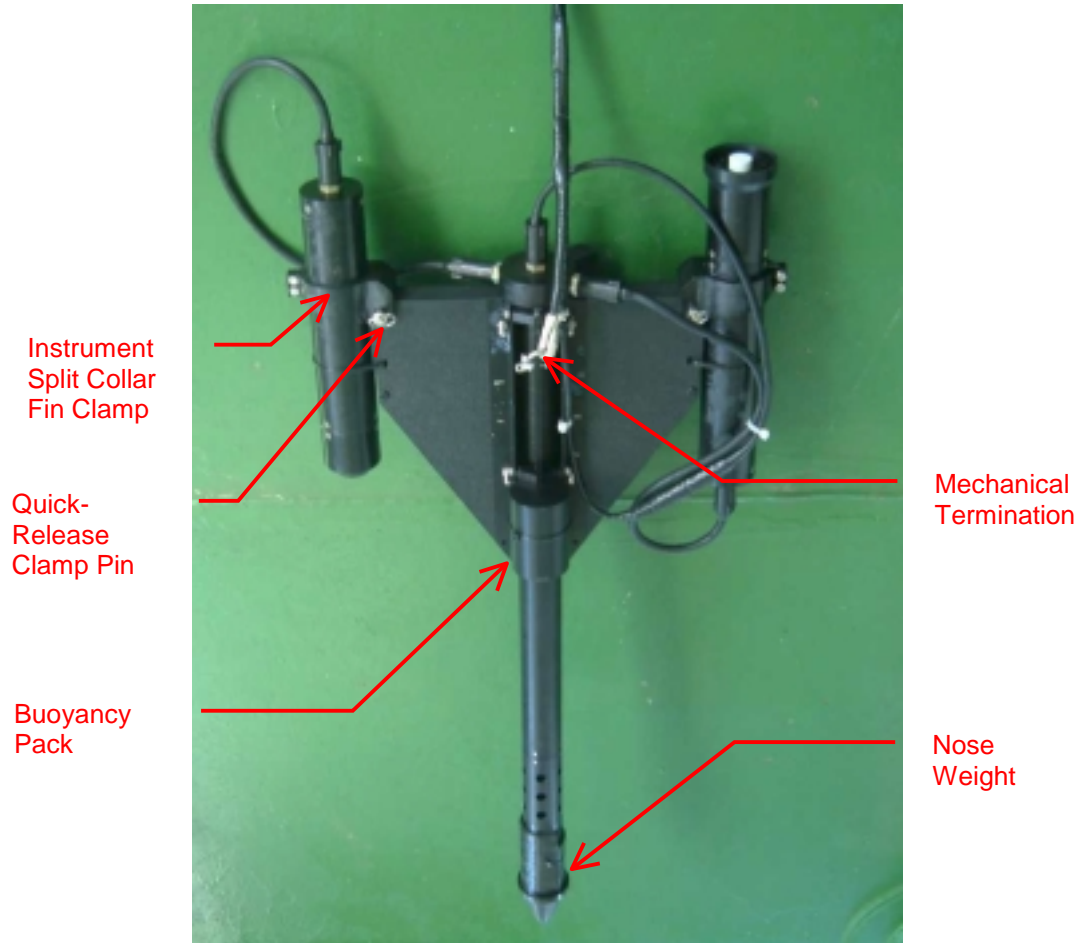
Figure C-1: HyperPro Assembly
