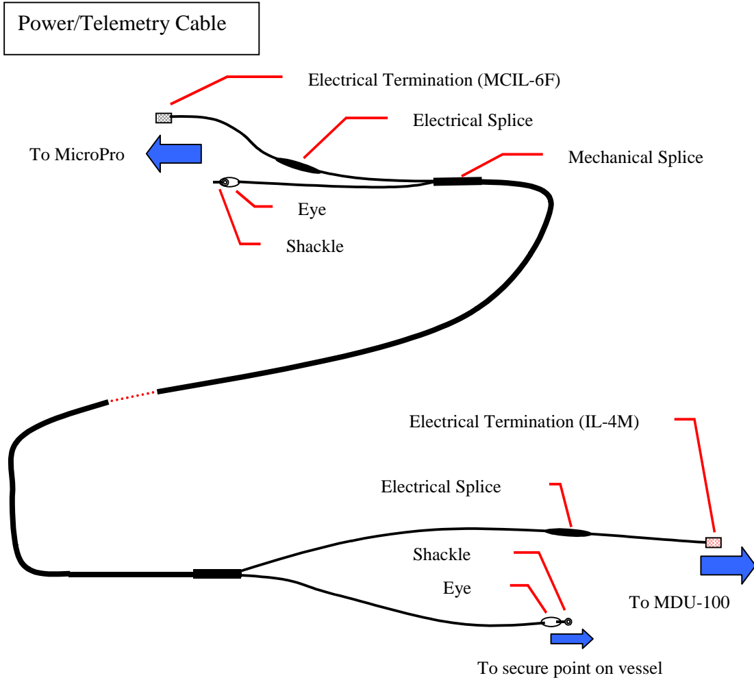
Figure C-3: Power/Telemetry Cable Connections
