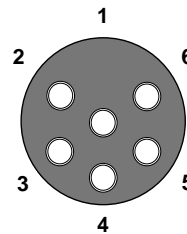
Figure A -A-7: MCBH-6-F Female Face View
