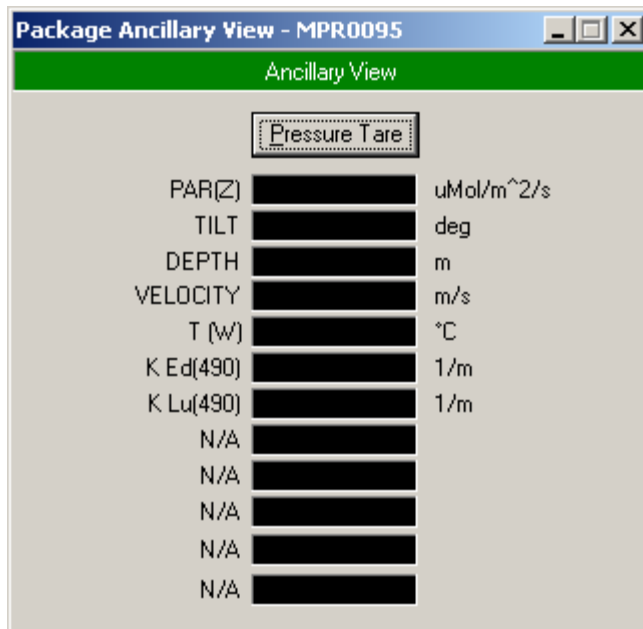
Figure D-4: Pressure Tare in SatView
