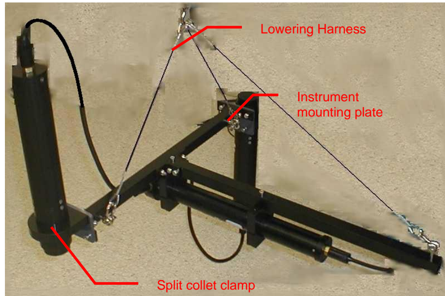
Figure C-1: Frame-mounted assembly
