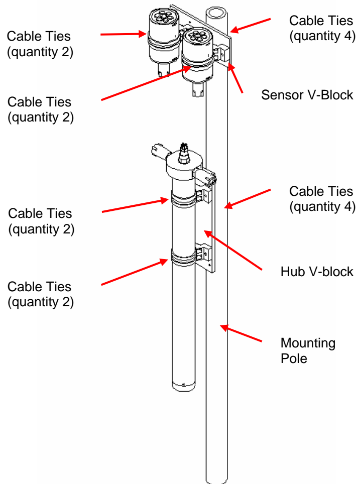
Figure C-7: Reference Sensor Mounting
