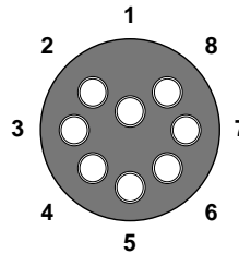
Figure A-5: MCBH-8-F Female Face View
