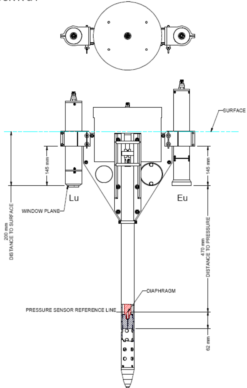
Figure C-4: Sensor Position Measurements: Profiler II with HyperOCRs in Surface Mode
