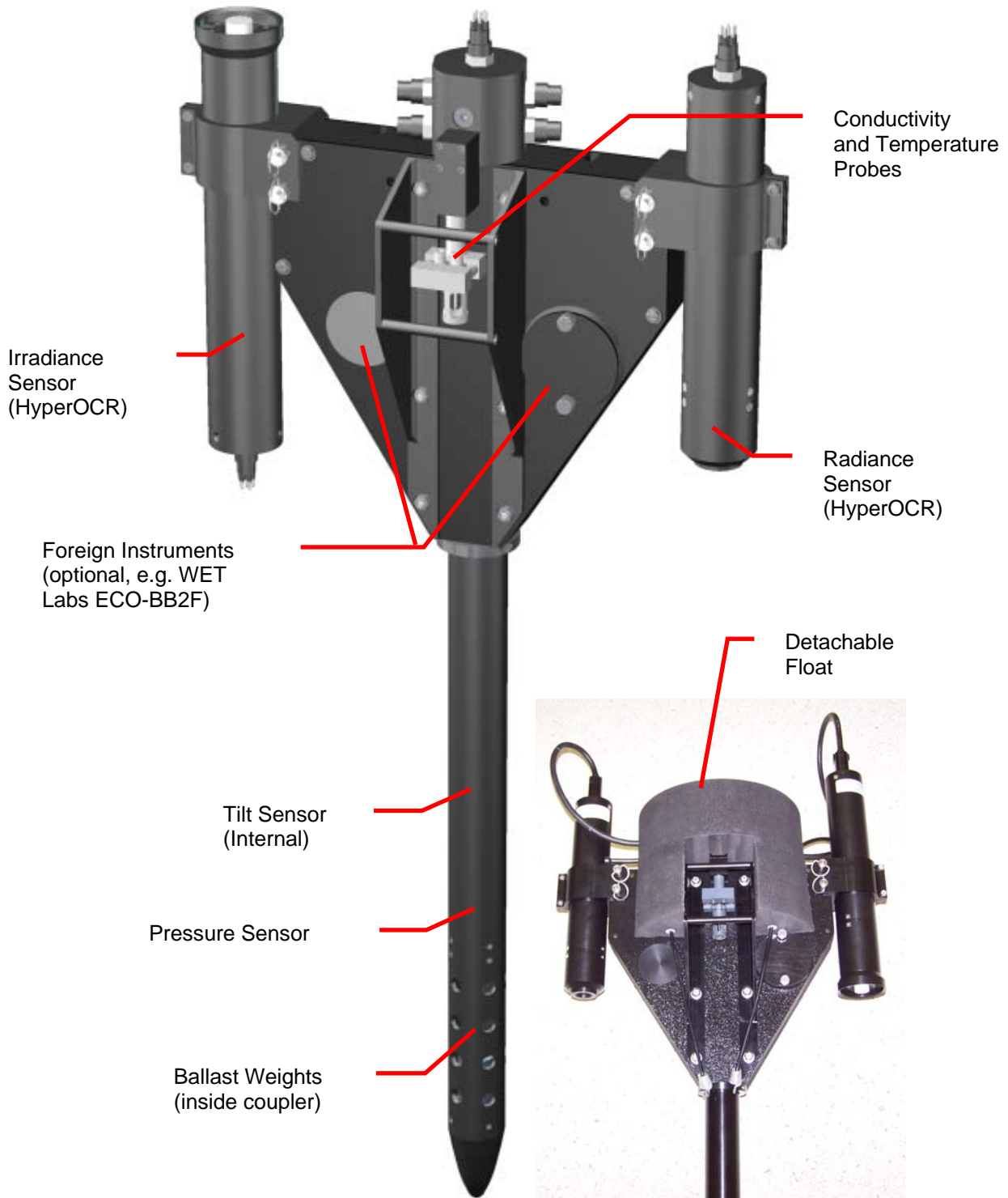
Figure A-3: Profiler II Major Components
