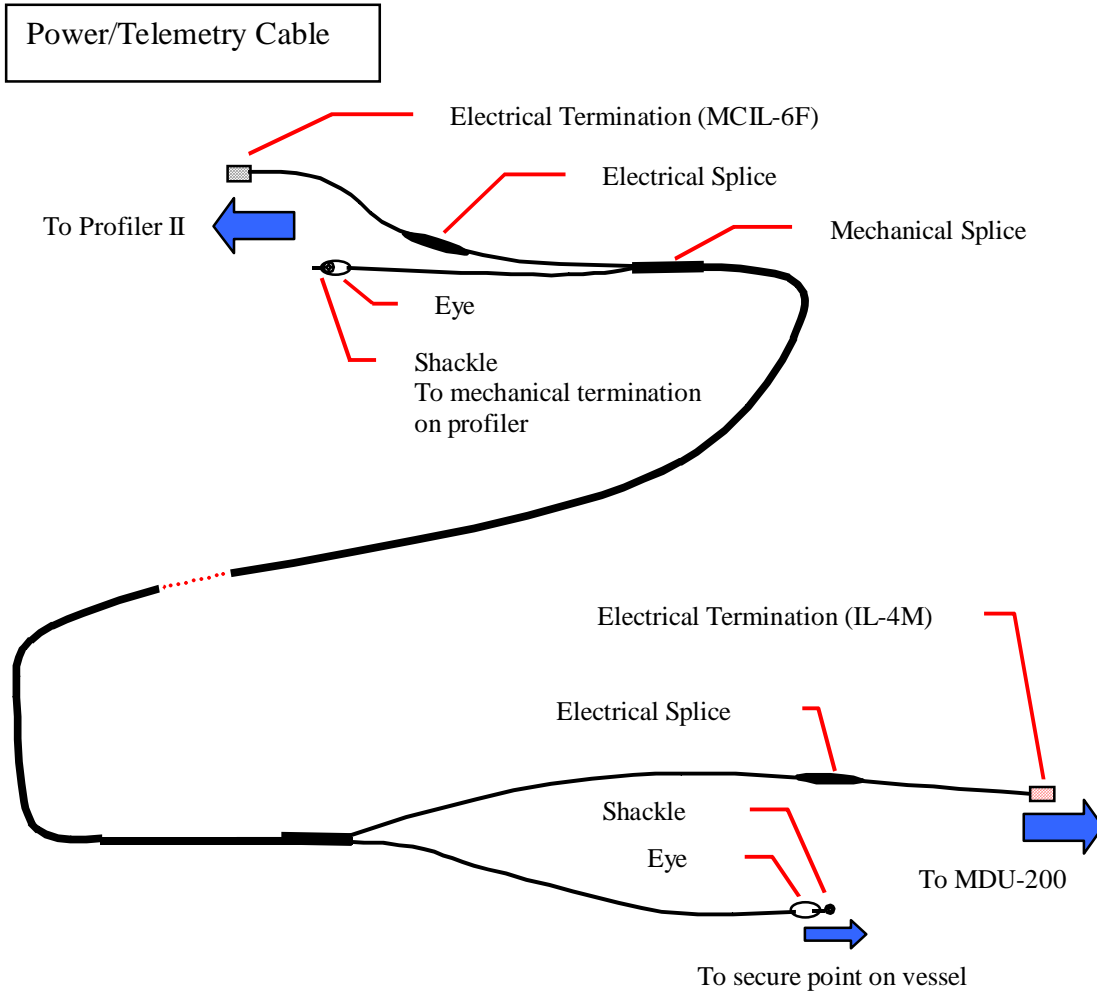
Figure C-2: Power/Telemetry Cable Connections
