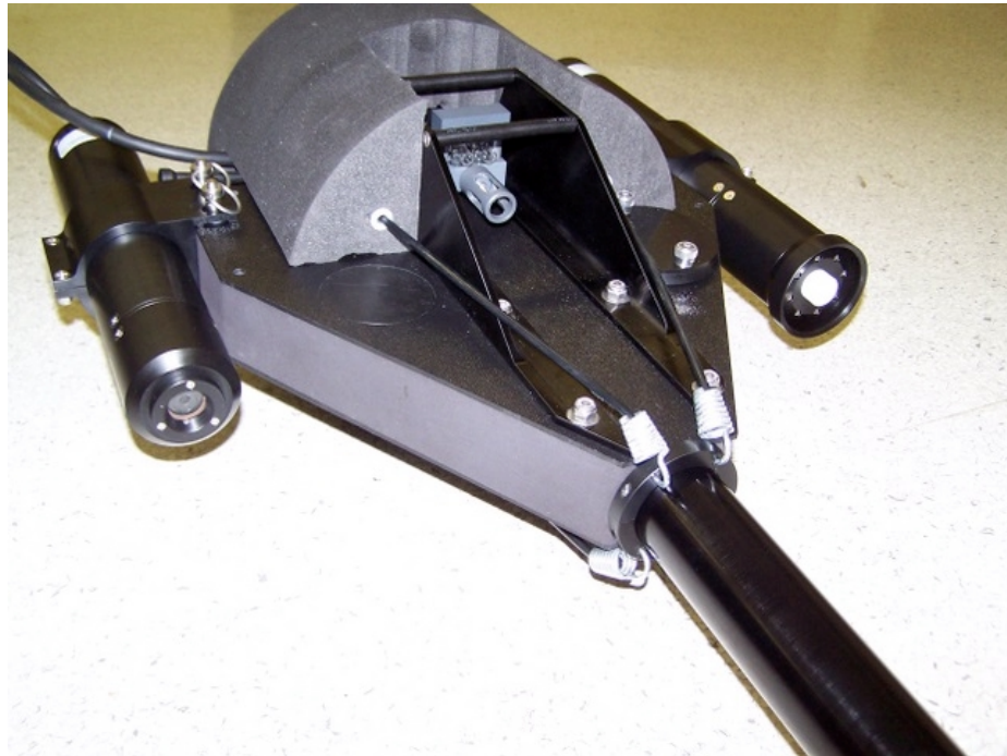
Figure D-5: Float installation for Profiler II Surface Mode
