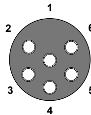
Figure A-7 MCBH-6-F Female Face View
