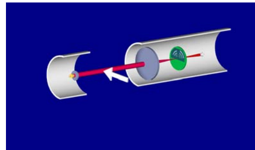
Figure 2: This is the LISST-100 . A collimated laser beam emanates from left. Particles in the flow scatter light. A receiving lens collects the scattered light, which is detected by the ring detector . A hole in the center of the ring detector permits the focused laser beam to pass through, where its power is sensed. This constitutes a transmission measurement. This measurement corrects for attenuation of the scattered light that is sensed by the rings.
