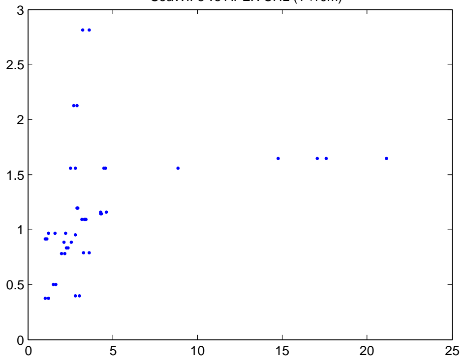
SeaWIFs vs APEX CHL (1<10m)
