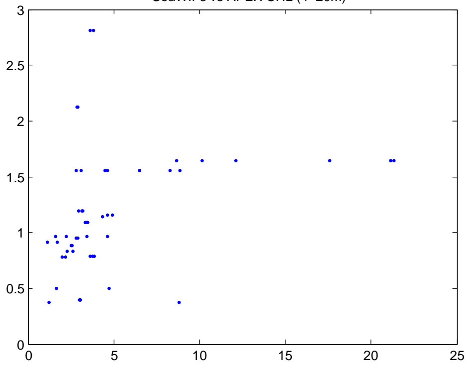
SeaWIFs vs APEX CHL (4–20m)
