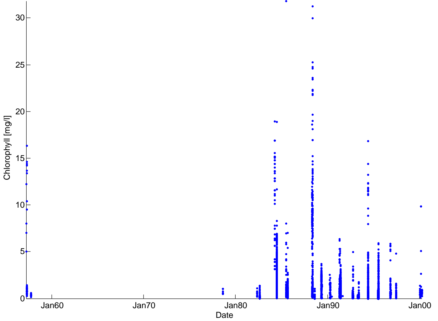
WOD01 OSD Data Chlorophyll vs. Date
