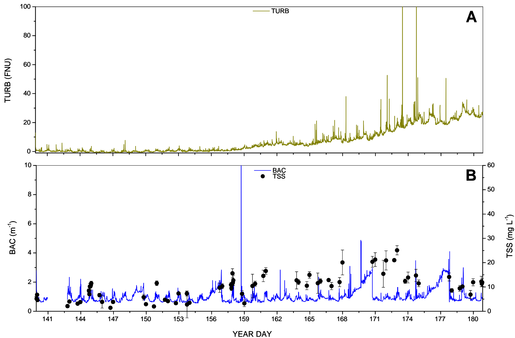
Figure 13. Kaneohe Bay, HI. A) Turbidity (TURB; Formazin Nephelometric Units) measured by the In-Situ Troll 9500; B) Beam Attenuation Coefficient (BAC) measured by an in situ transmissometer, and total suspended solids (TSS).
