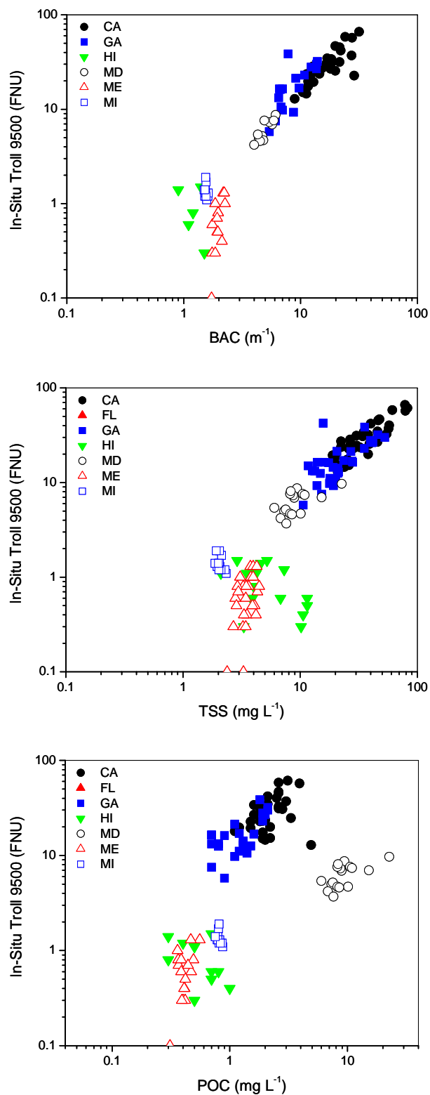
Figure 21. In-Situ Troll 9500 turbidity data (in Formazin Nephelometric Units) plotted against Beam Attenuation Coefficients (BAC), collected total suspended solids (TSS) and particulate organic carbon (POC).
