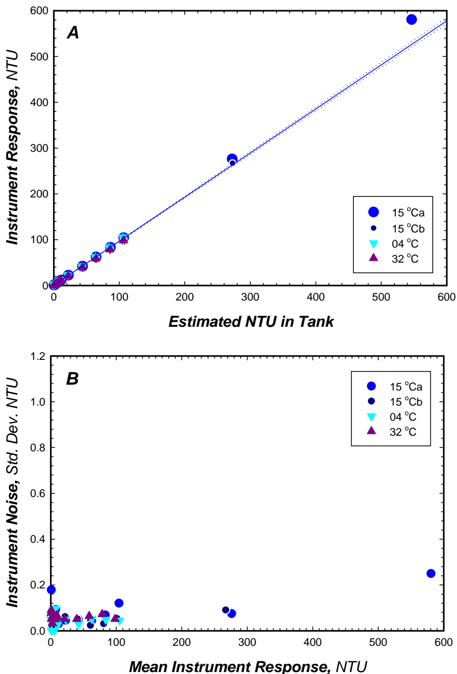
Figure 1. In-Situ's Troll 9500 signal and instrument noise in response to increasing turbidity derived from SDVB added to filtered deionized water at three test temperatures. (A) Mean detector response to sequential additions of known SDVB concentrations. Instrument response over a turbidity range normally observed in natural waters (0-100 NTU) was modeled by linear regression. Modeled response at 15°C, with 99% confidence intervals (dotted lines): NTU_{instru} = 0.962NTU_{SDVB} + 0.691 , r^2 = 0.999 , demonstrates response is linear through 280 NTU SDVB. Detector response was unaffected by the ambient temperatures tested. (B) Signal noise (s.d.) ranged from <0.1 to 10% of measured signal in the presence of SDVB and no consistent temperature or turbidity dependence was detected.
