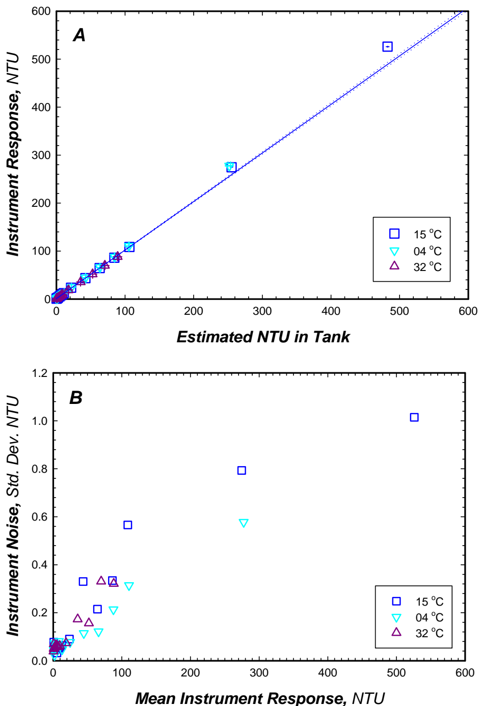
Figure 2. In-Situ's Troll 9500 signal and instrument noise in response to increasing turbidity derived from Formazin added to filtered deionized water at three test temperatures. (A) Mean detector response to sequential additions of known Formazin concentrations. Instrument response over a turbidity range normally observed in natural waters (0-100 NTU) was modeled by linear regression. Modeled response at 15°C, with 99% confidence intervals (dotted lines): NTU_{instru} = 1.012NTU_{FRMZ} + 1.004 , r^2 = 0.999 , demonstrates response is linear through at least 260 NTU Frmz. Detector response was unaffected by the ambient temperatures tested. (B) Signal noise (s.d.) ranged from 0.2 to 7% of measured signal and was independent of temperature. The increase in signal s.d. with Formazin turbidity, likely results from detection of particle aggregates in suspension.
