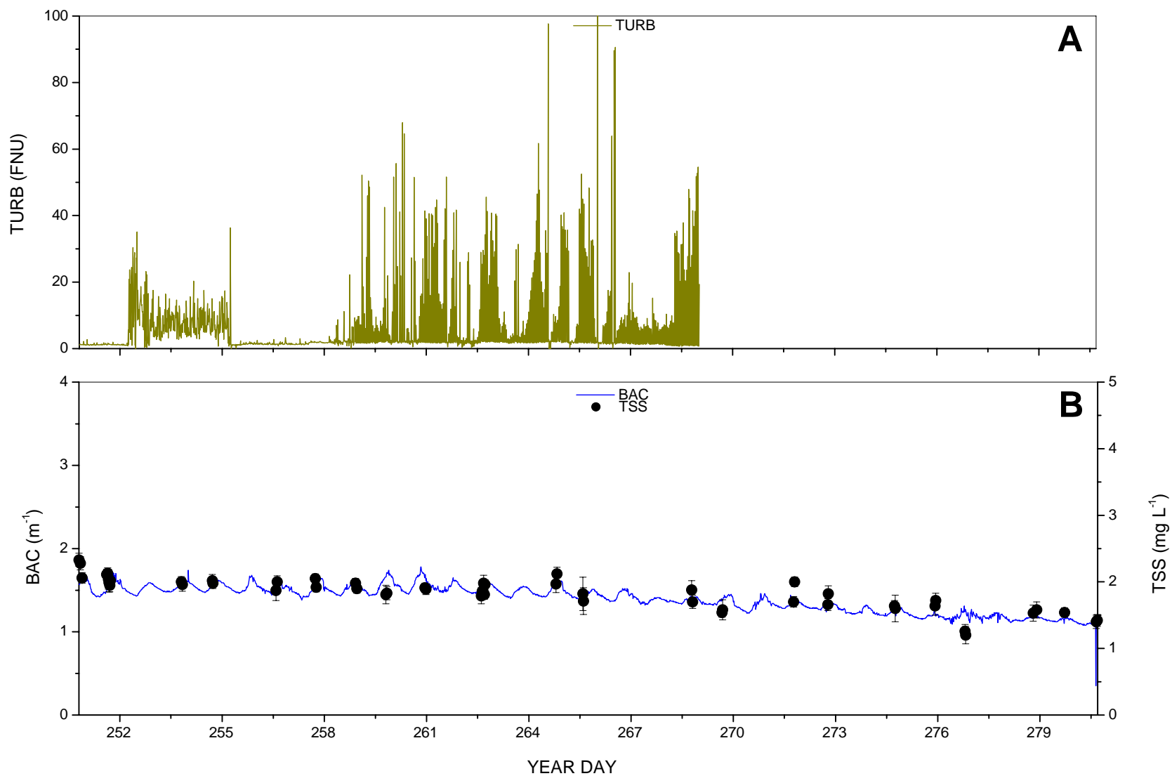
Figure 19. Winans Lake, MI. A) Turbidity (TURB; Formazin Nephelometric Units) measured by the In-Situ Troll 9500; B) Beam Attenuation Coefficient (BAC) measured by an in situ transmissometer, and total suspended solids (TSS).
