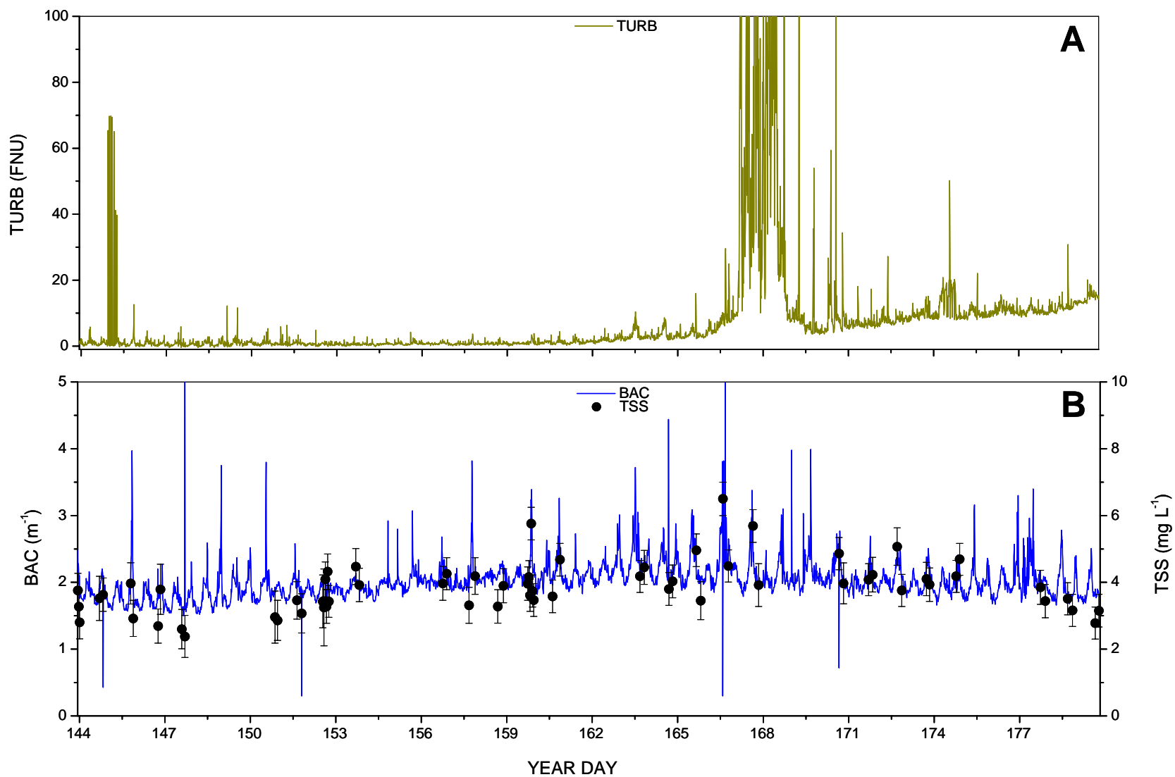
Figure 17. Damariscotta River Estuary, ME. A) Turbidity (TURB: Nephelometric Units) measured by the In-Situ Troll 9500; B) Beam Attenuation Coefficient (BAC) measured by an in situ transmissometer, and total suspended solids (TSS).
