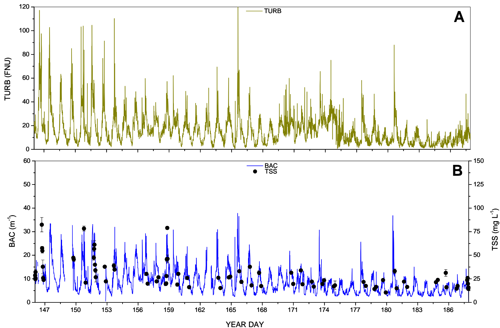
Figure 7. Moss Landing Harbor, CA. A) Turbidity (TURB; Formazin Nephelometric Units) measured by the In-Situ Troll 9500; B) Beam Attenuation Coefficient (BAC) measured by an in situ transmissometer, and total suspended solids (TSS).
