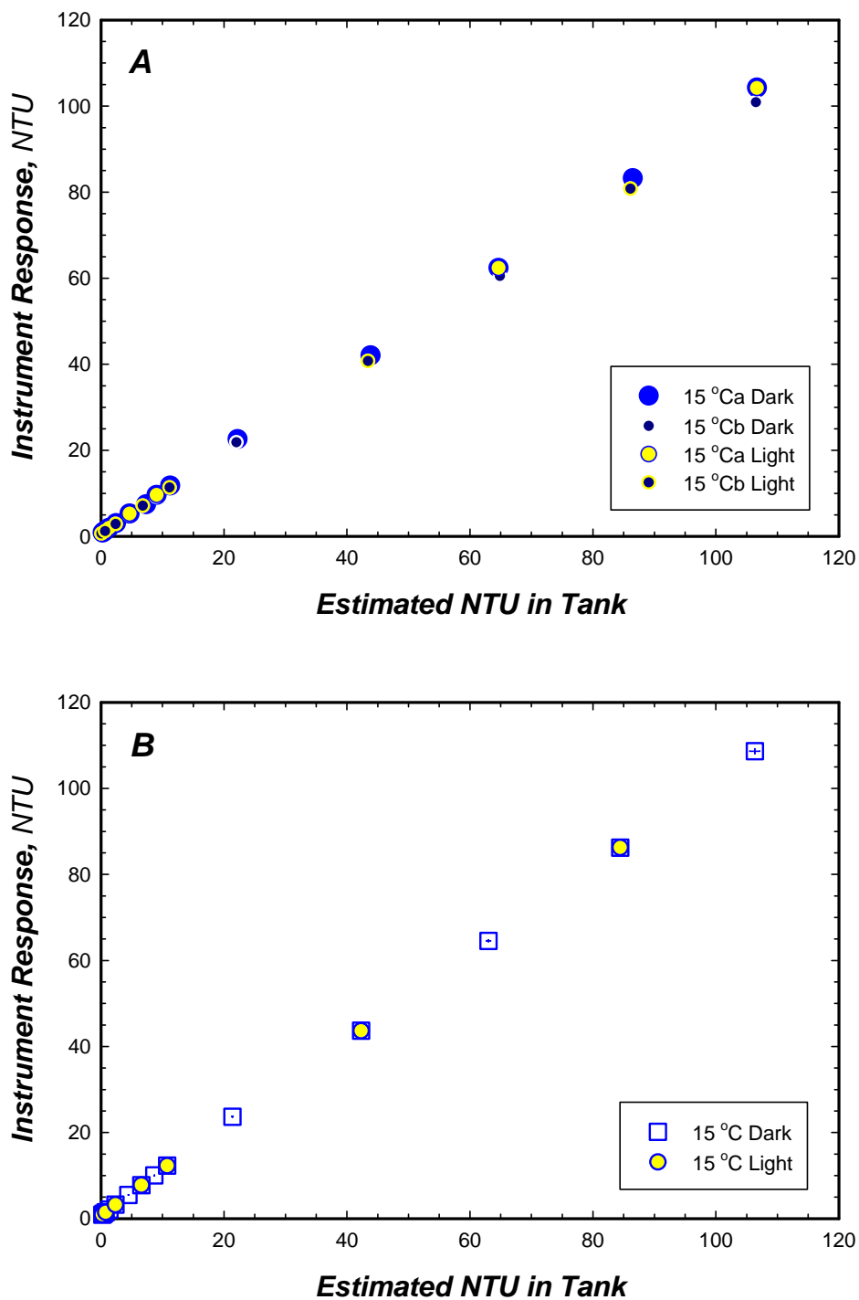
Figure 3. Effects of down-welling irradiance on turbidity measurement by the In-Situ Troll 9500 turbidity sensor. Surface irradiance applied at each indicated test concentration using a bank of three 500W halogen lamps. E_0 : 400-500 \mu\text{mol quanta m}^{-2} \text{s}^{-1} measured using a Licor 190S detector. (A) Mean detector response to sequential additions of known SDVB concentrations. (B) Mean detector response to sequential additions of known Formazin concentrations. Exposure to down-welling irradiance did not have a significant impact on instrument response under these test conditions.
