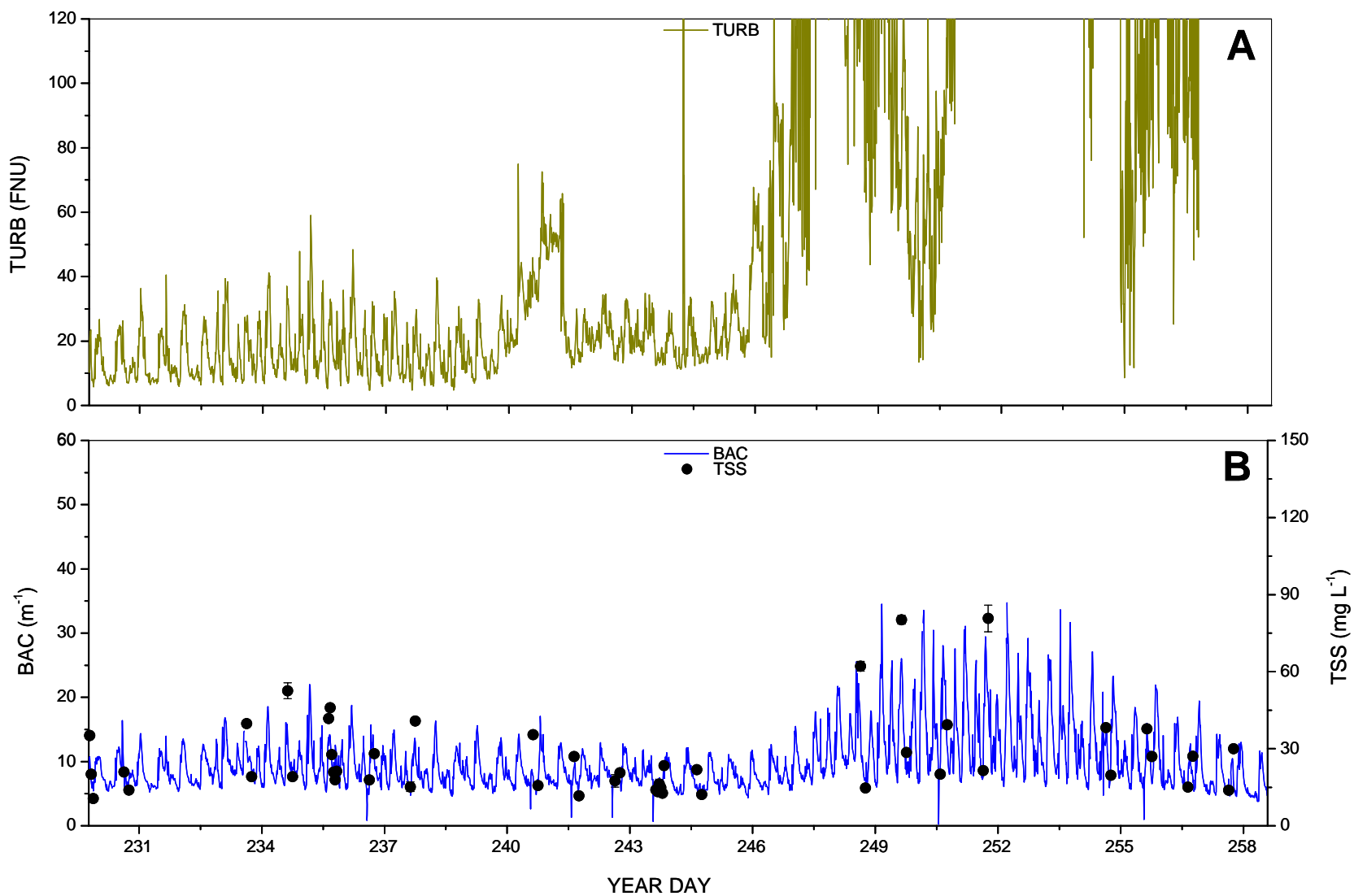
Figure 11. Skidaway Island, GA. A) Turbidity (TURB; Formazin Nephelometric Units) measured by the In-Situ Troll 9500; B) Beam Attenuation Coefficient (BAC) measured by an in situ transmissometer, and total suspended solids (TSS).
