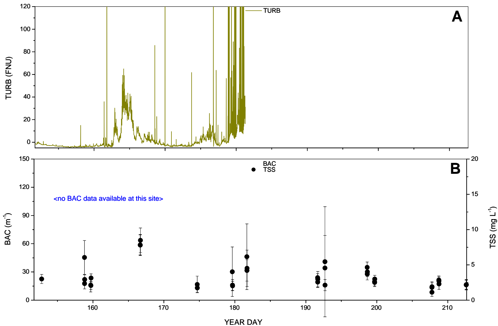
Figure 9. Offshore of Tampa Bay, FL. A) Turbidity (TURB; Formazin Nephelometric Units) measured by the In-Situ Troll 9500; B) Beam Attenuation Coefficient (BAC) measured by an in situ transmissometer, and total suspended solids (TSS).
