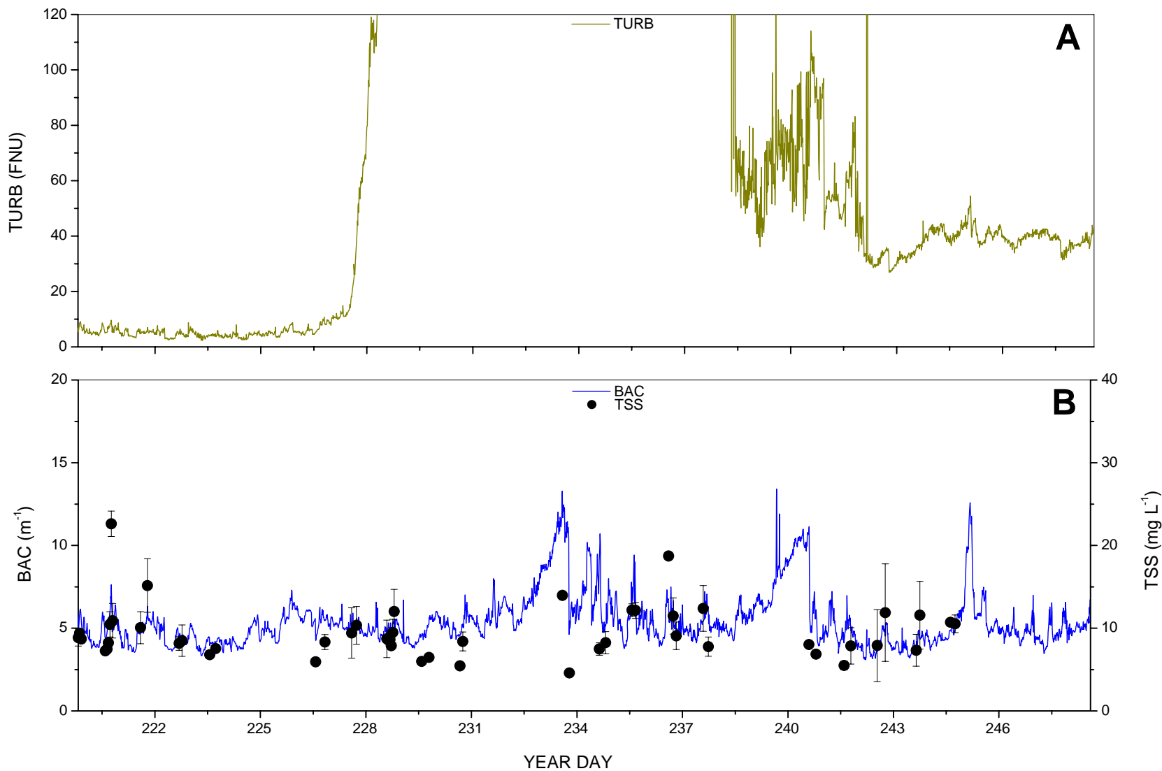
Figure 15. Chesapeake Bay, MD. A) Turbidity (TURB; Formazin Nephelometric Units) measured by the In-Situ Troll 9500; B) Beam Attenuation Coefficient (BAC) measured by an in situ transmissometer, and total suspended solids (TSS).
